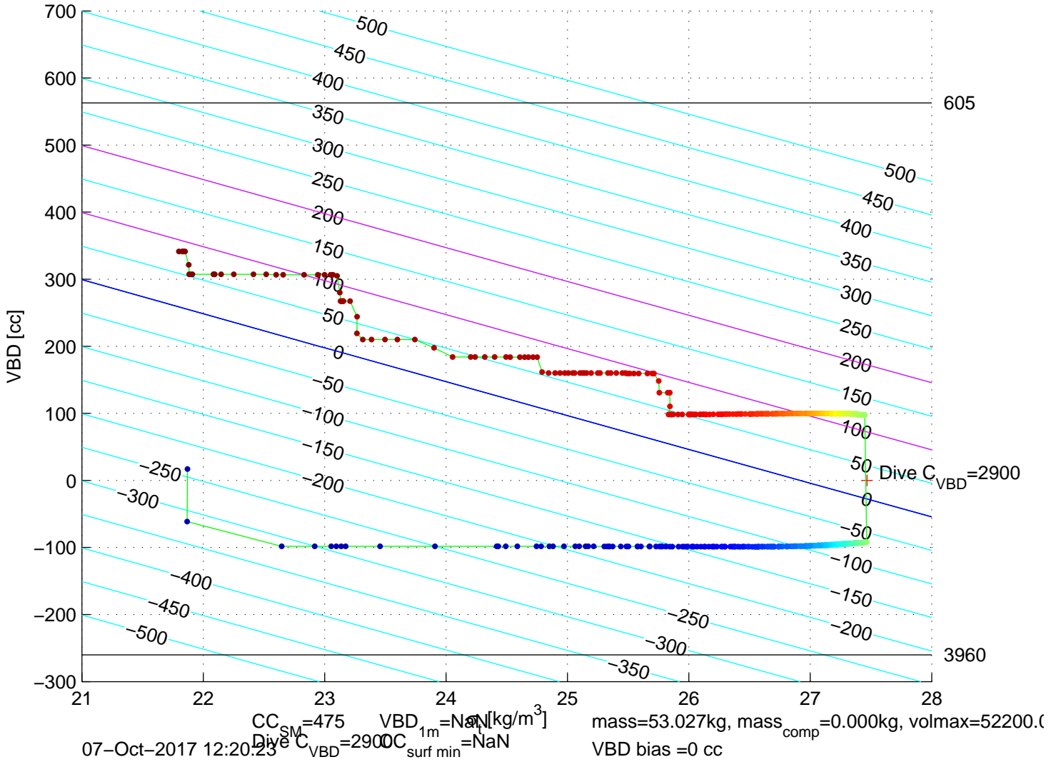
p6300658: SG630 Mission 7 Jul 2017 07–Oct–2017 11:32:00Z – buoyancy contoured
