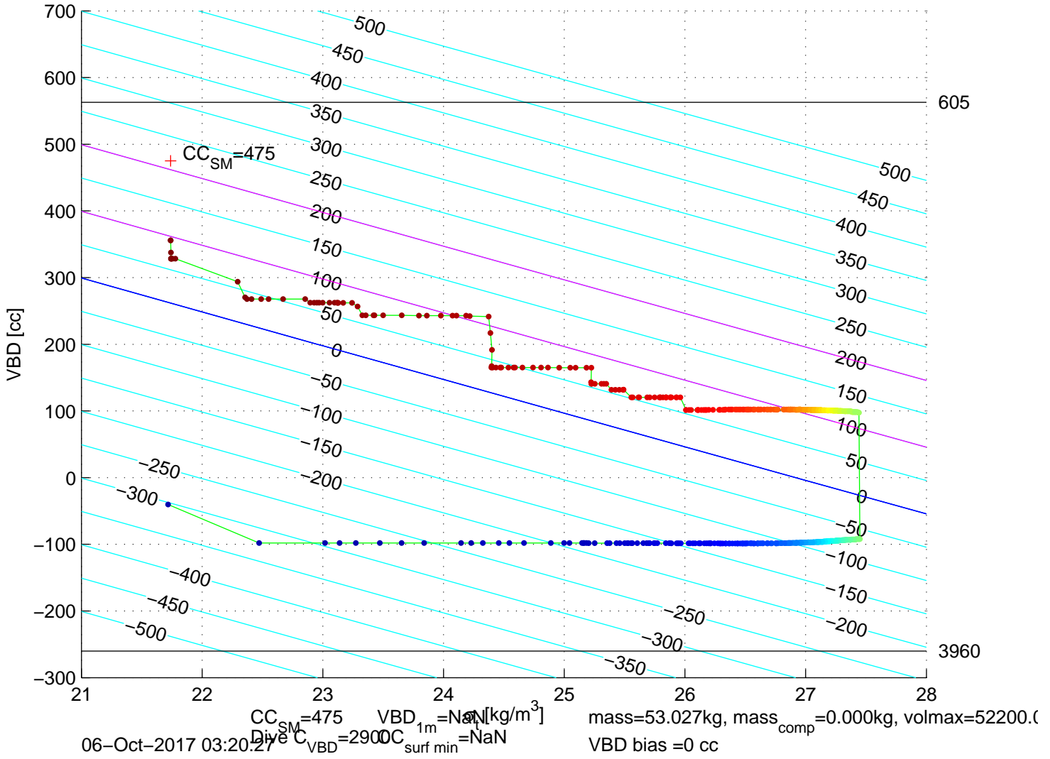
p6300651: SG630 Mission 7 Jul 2017 06–Oct–2017 02:28:14Z – buoyancy contoured
