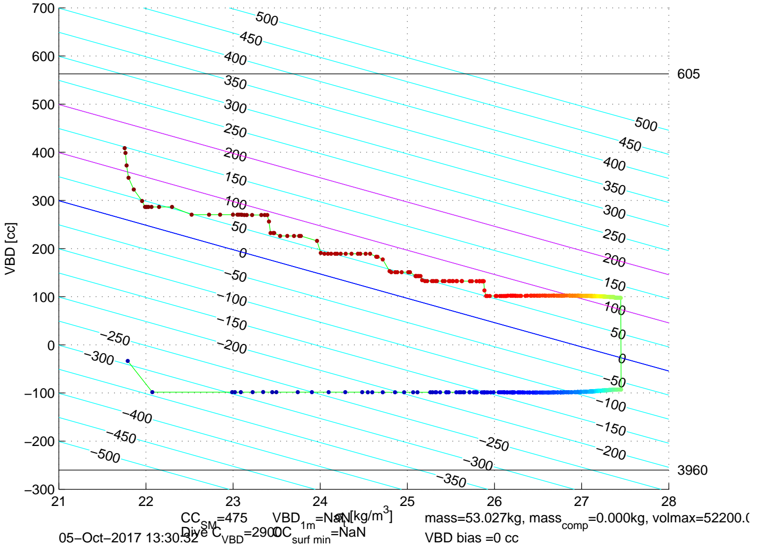
p6300648: SG630 Mission 7 Jul 2017 05–Oct–2017 12:41:58Z – buoyancy contoured
