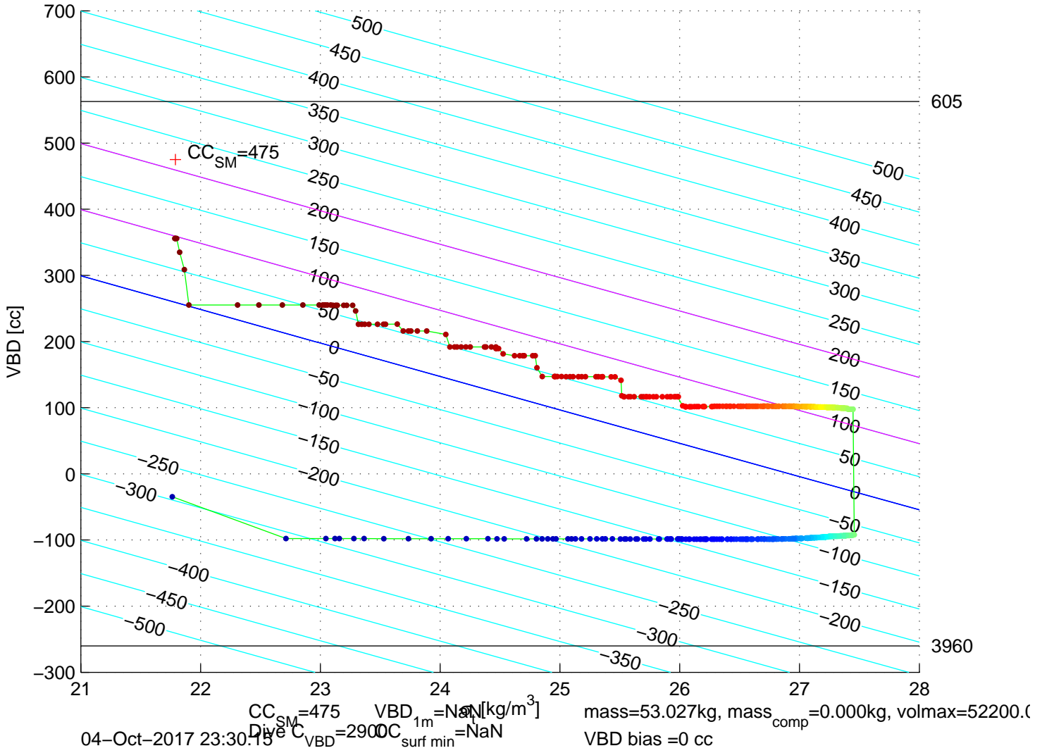
p6300645: SG630 Mission 7 Jul 2017 04–Oct–2017 22:42:54Z – buoyancy contoured
