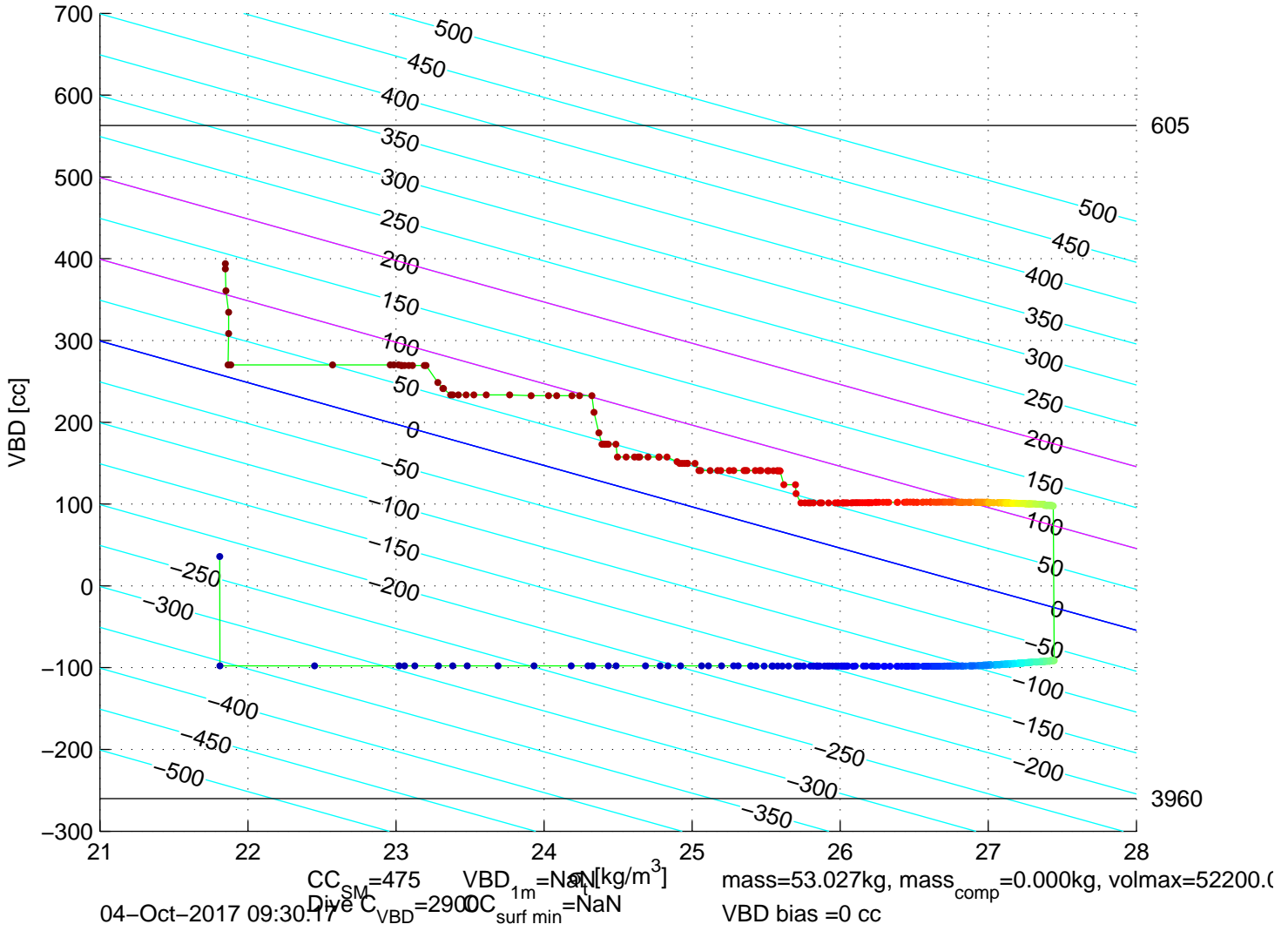
p6300642: SG630 Mission 7 Jul 2017 04–Oct–2017 08:35:05Z – buoyancy contoured
