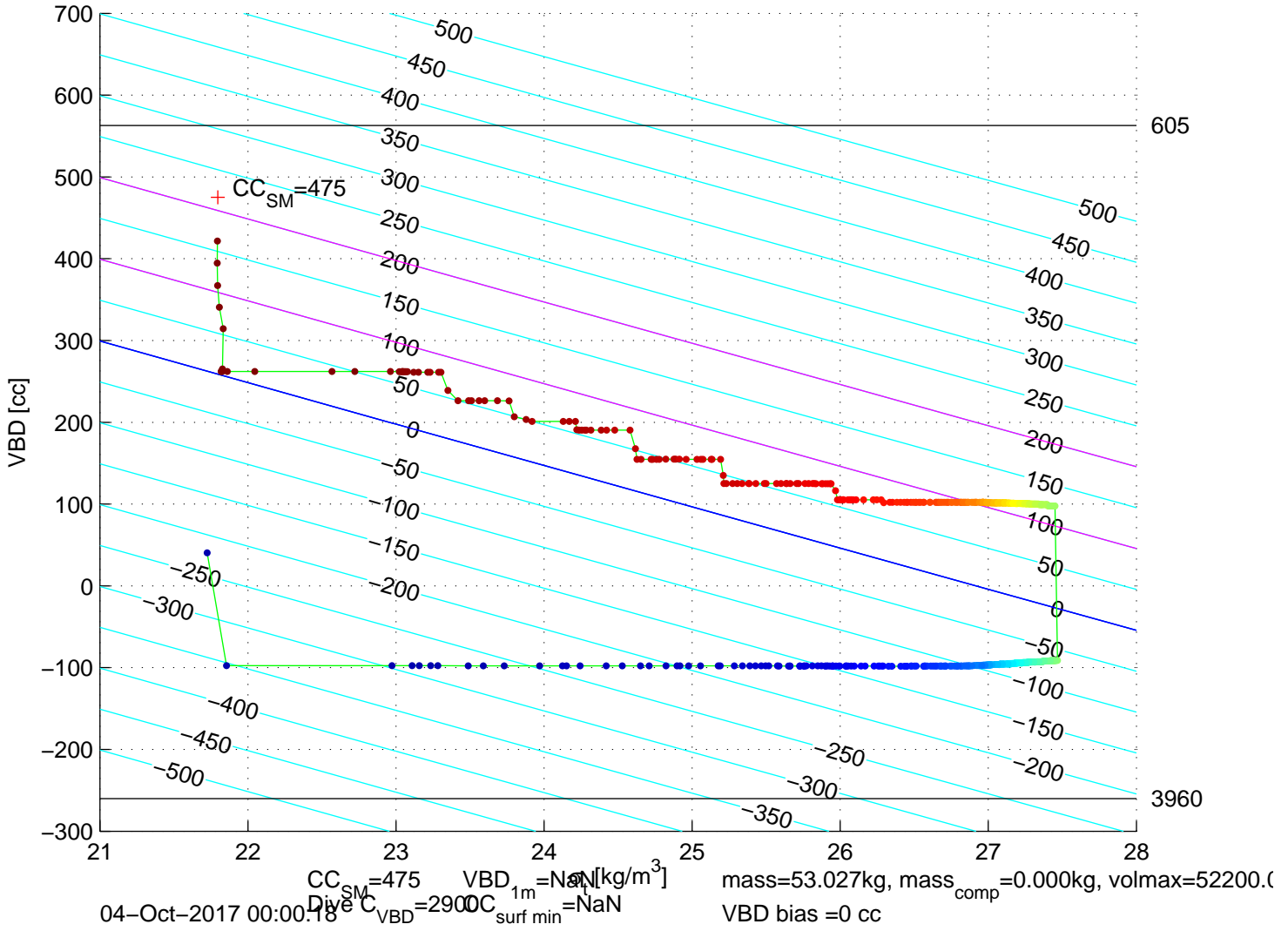
p6300640: SG630 Mission 7 Jul 2017 03–Oct–2017 23:05:34Z – buoyancy contoured
