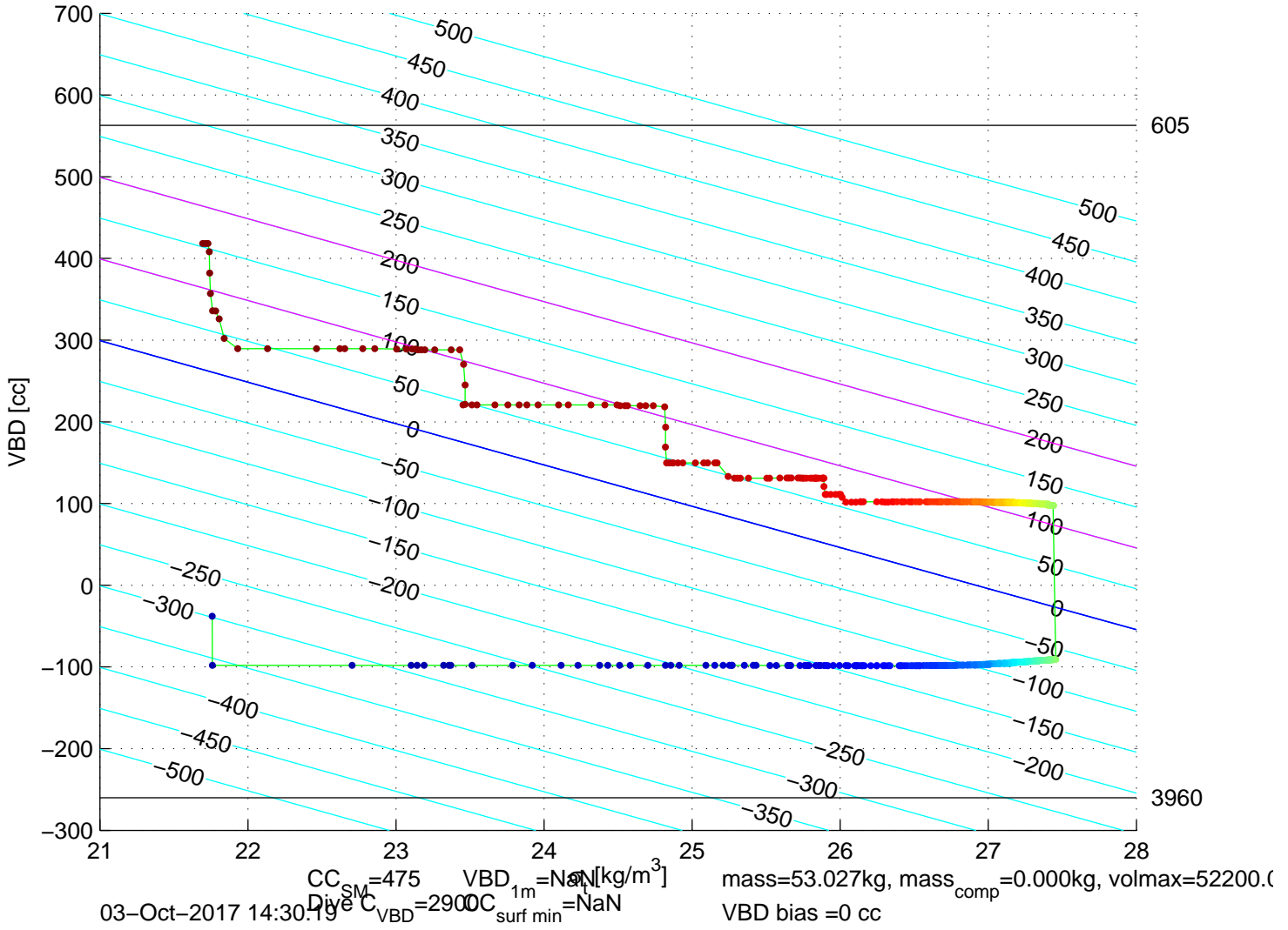
p6300638: SG630 Mission 7 Jul 2017 03–Oct–2017 13:40:23Z – buoyancy contoured
