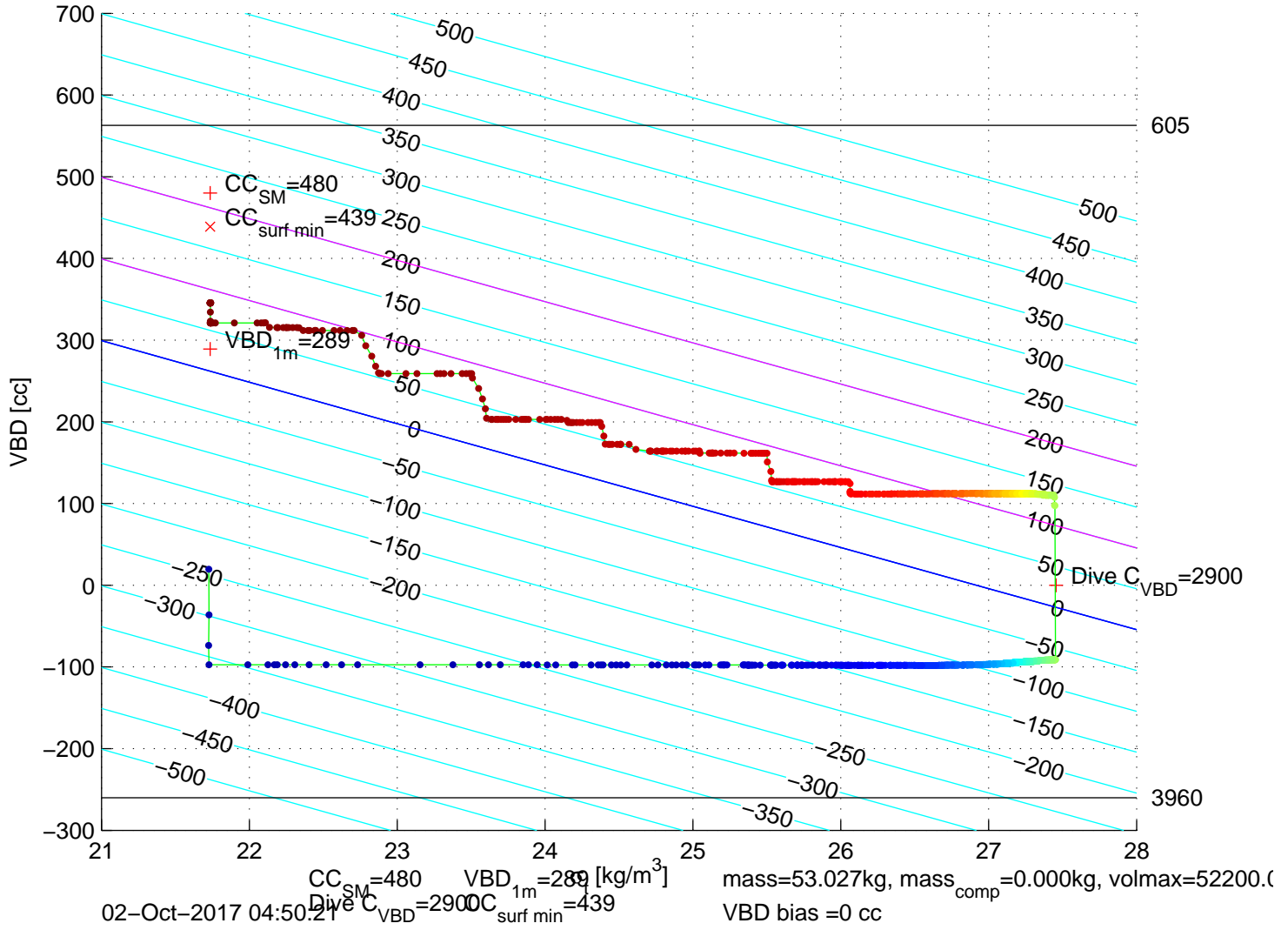
p6300631: SG630 Mission 7 Jul 2017 02–Oct–2017 04:11:21Z – buoyancy contoured
