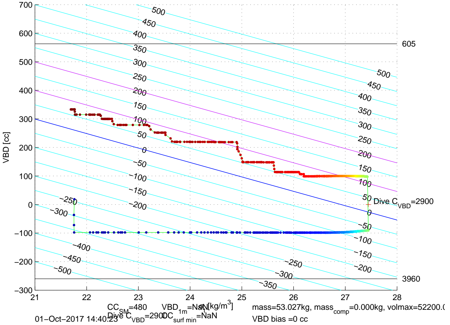
p6300628: SG630 Mission 7 Jul 2017 01–Oct–2017 13:46:35Z – buoyancy contoured
