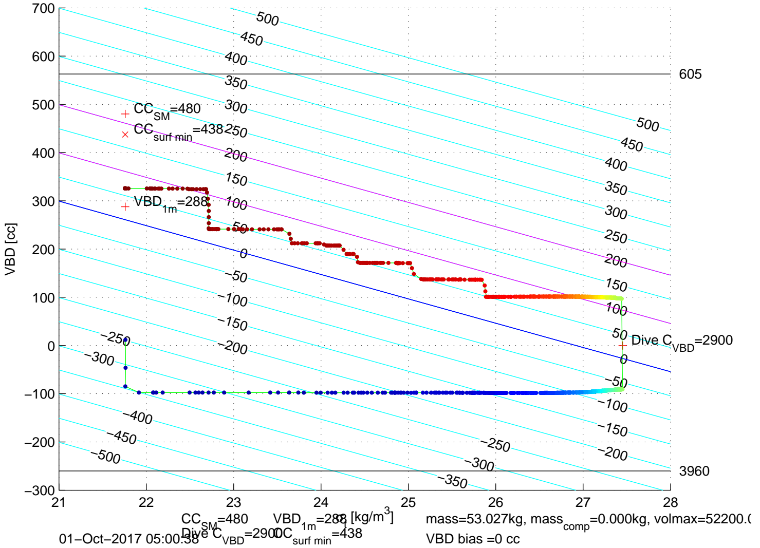
p6300626: SG630 Mission 7 Jul 2017 01–Oct–2017 04:07:58Z – buoyancy contoured
