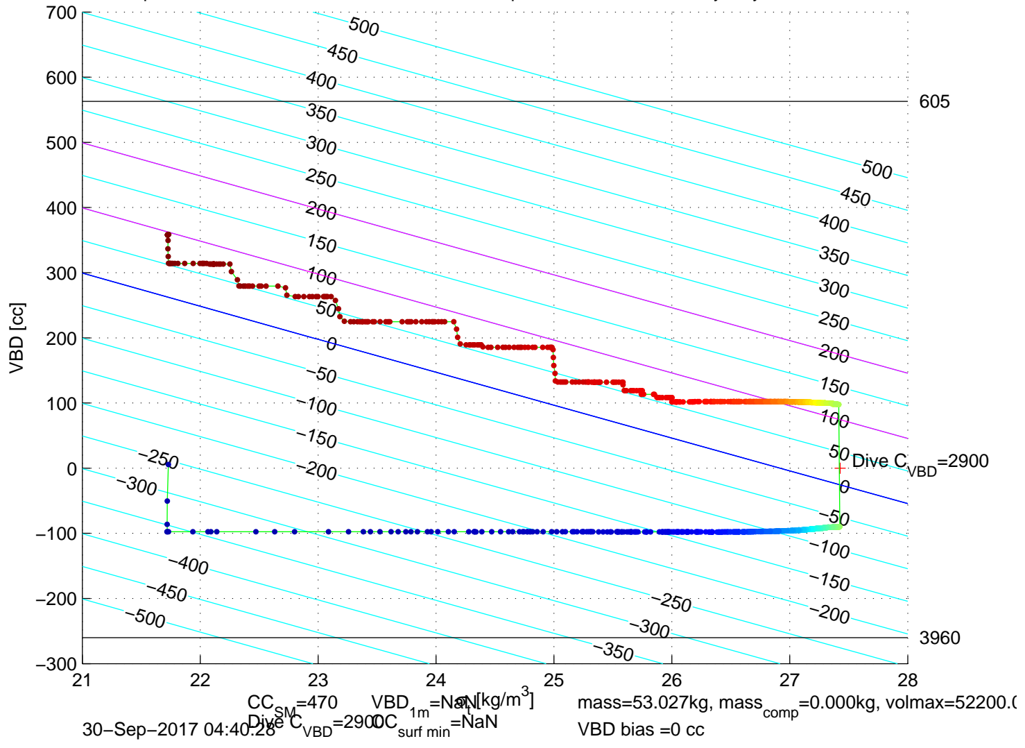
p6300621: SG630 Mission 7 Jul 2017 30-Sep-2017 03:45:10Z – buoyancy contoured
