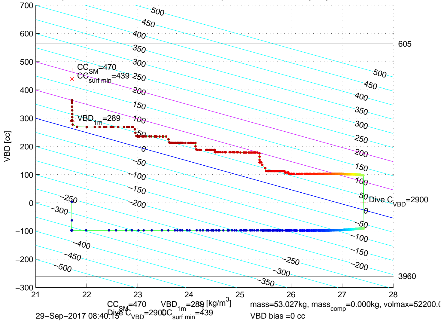
p6300617: SG630 Mission 7 Jul 2017 29-Sep-2017 07:48:27Z – buoyancy contoured
