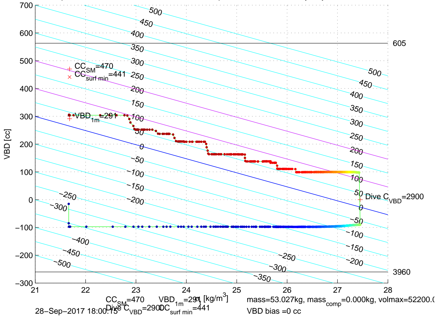
p6300614: SG630 Mission 7 Jul 2017 28-Sep-2017 17:15:36Z – buoyancy contoured
