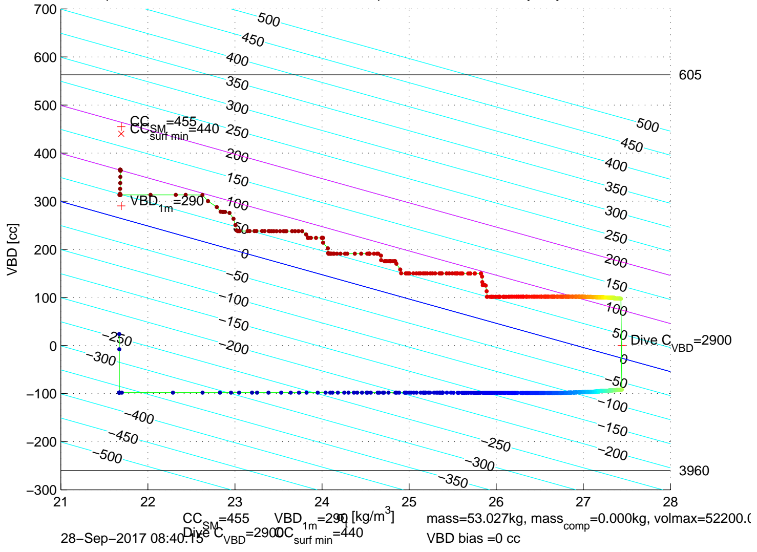
p6300612: SG630 Mission 7 Jul 2017 28-Sep-2017 07:57:51Z – buoyancy contoured
