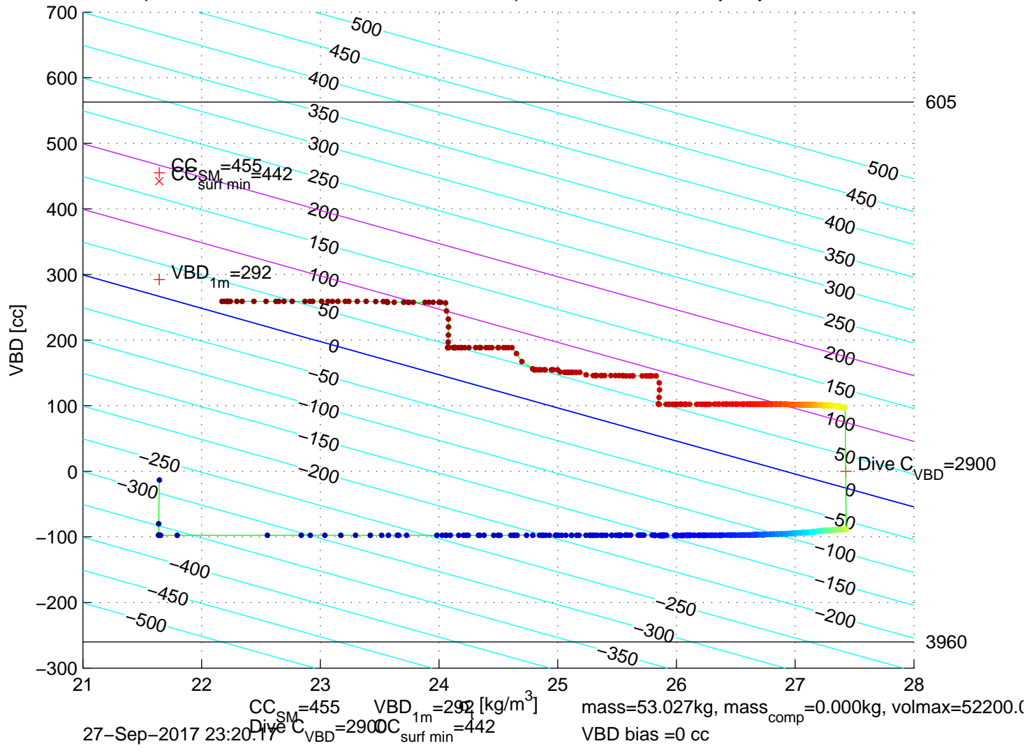
p6300610: SG630 Mission 7 Jul 2017 27-Sep-2017 22:36:40Z – buoyancy contoured
