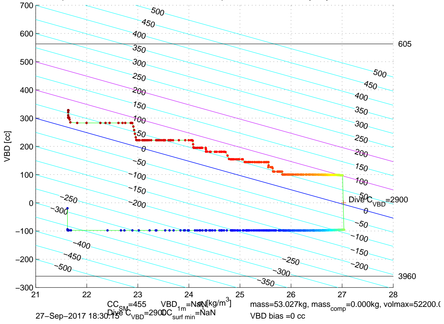
p6300609: SG630 Mission 7 Jul 2017 27-Sep-2017 19:43:16Z – buoyancy contoured
