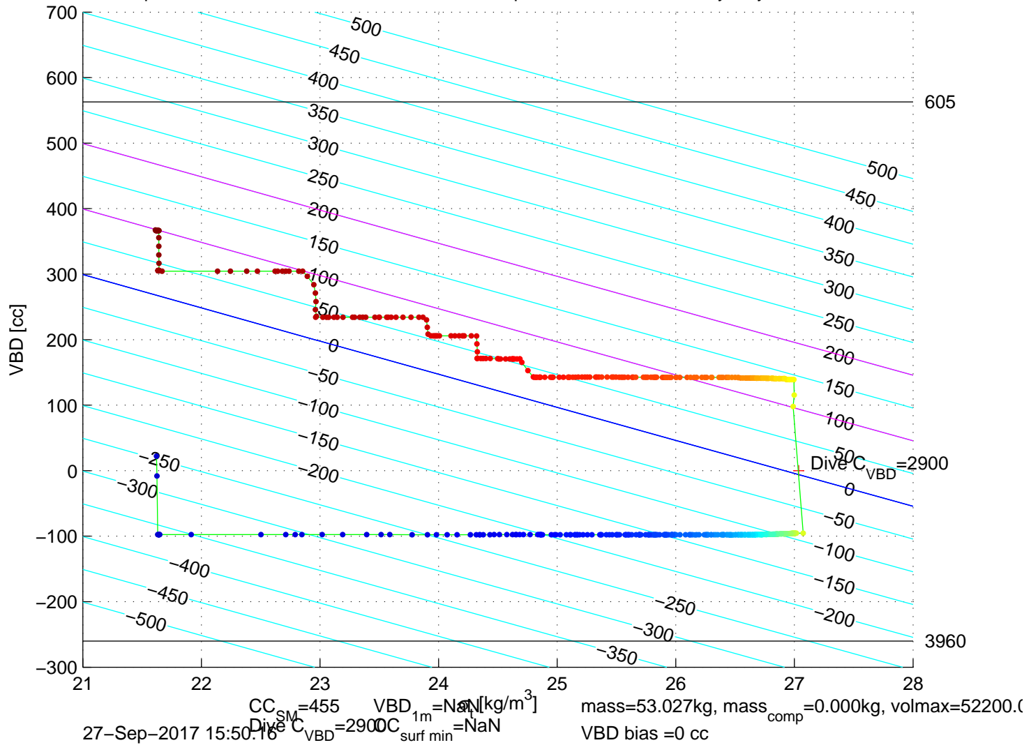
p6300608: SG630 Mission 7 Jul 2017 27-Sep-2017 17:10:32Z – buoyancy contoured
