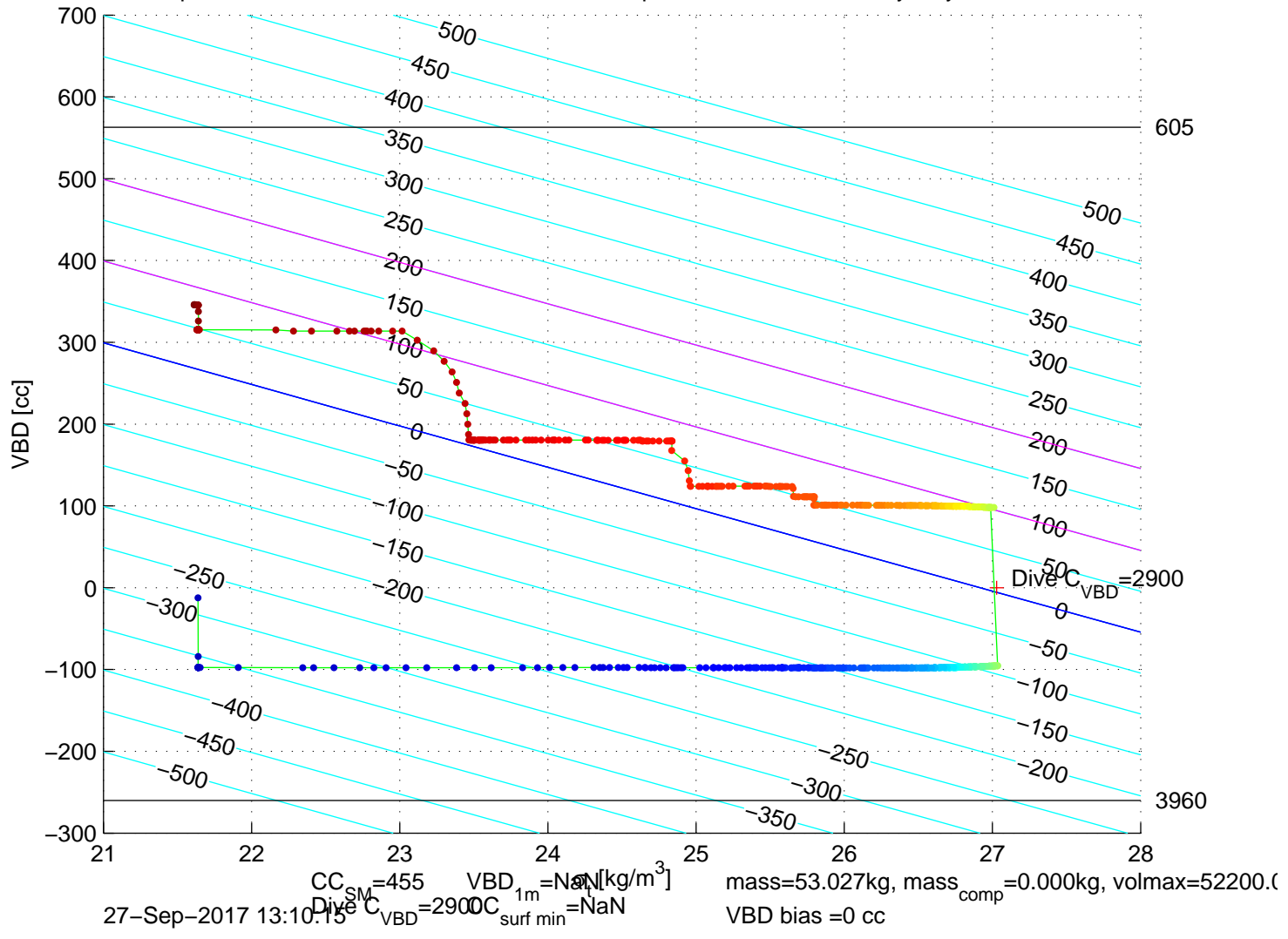
p6300607: SG630 Mission 7 Jul 2017 27-Sep-2017 14:26:05Z – buoyancy contoured
