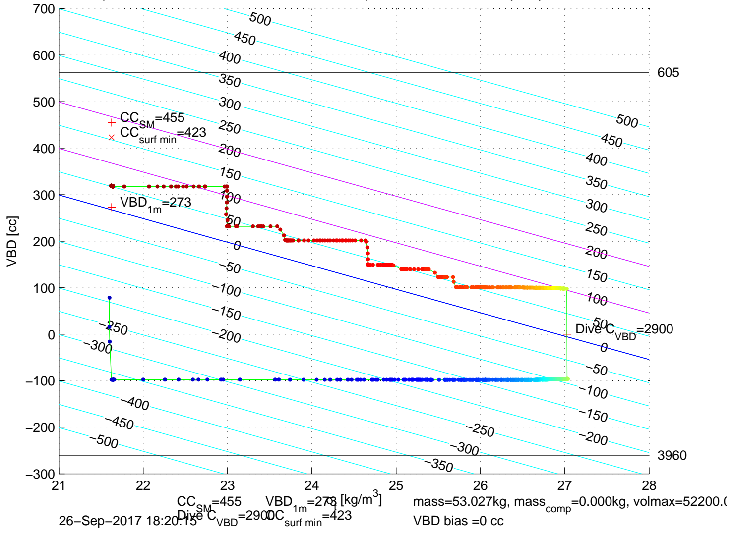
p6300600: SG630 Mission 7 Jul 2017 26-Sep-2017 19:40:03Z – buoyancy contoured
