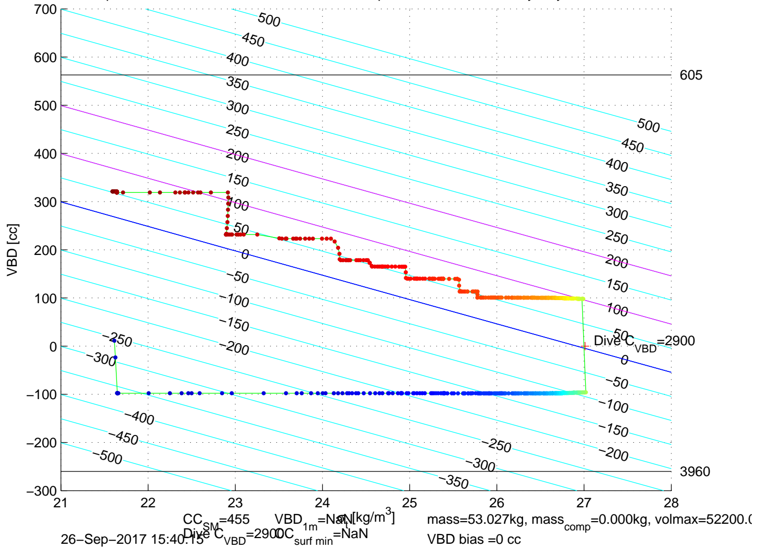
p6300599: SG630 Mission 7 Jul 2017 26-Sep-2017 17:02:32Z – buoyancy contoured
