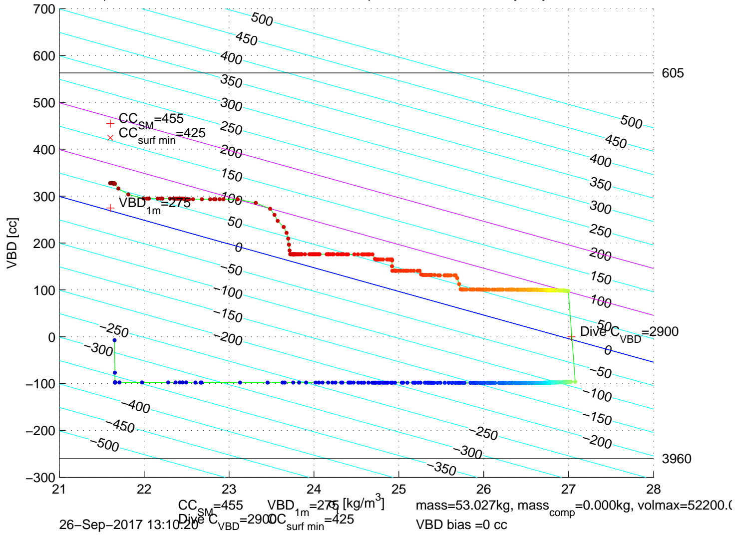
p6300598: SG630 Mission 7 Jul 2017 26-Sep-2017 14:25:25Z – buoyancy contoured
