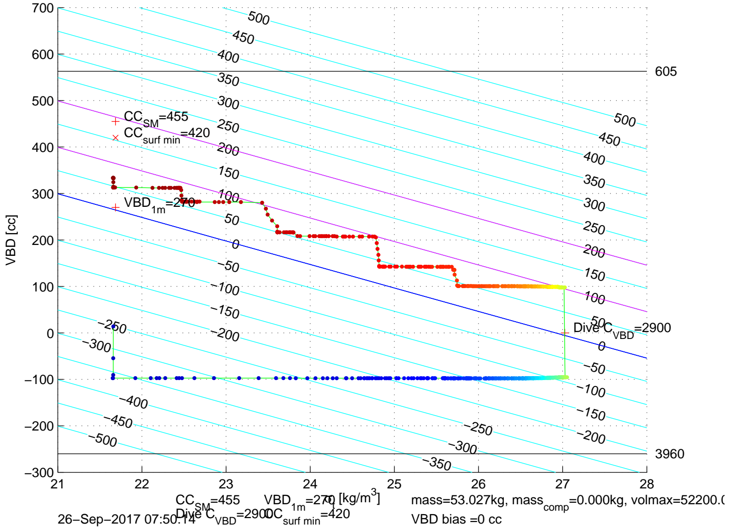
p6300596: SG630 Mission 7 Jul 2017 26-Sep-2017 09:03:17Z – buoyancy contoured
