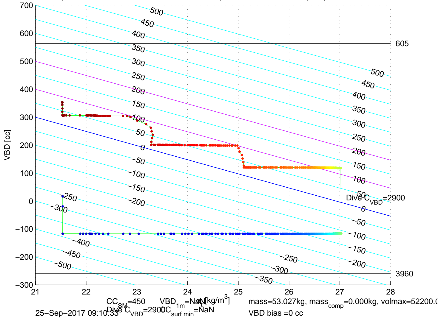
p6300587: SG630 Mission 7 Jul 2017 25-Sep-2017 10:46:14Z – buoyancy contoured
