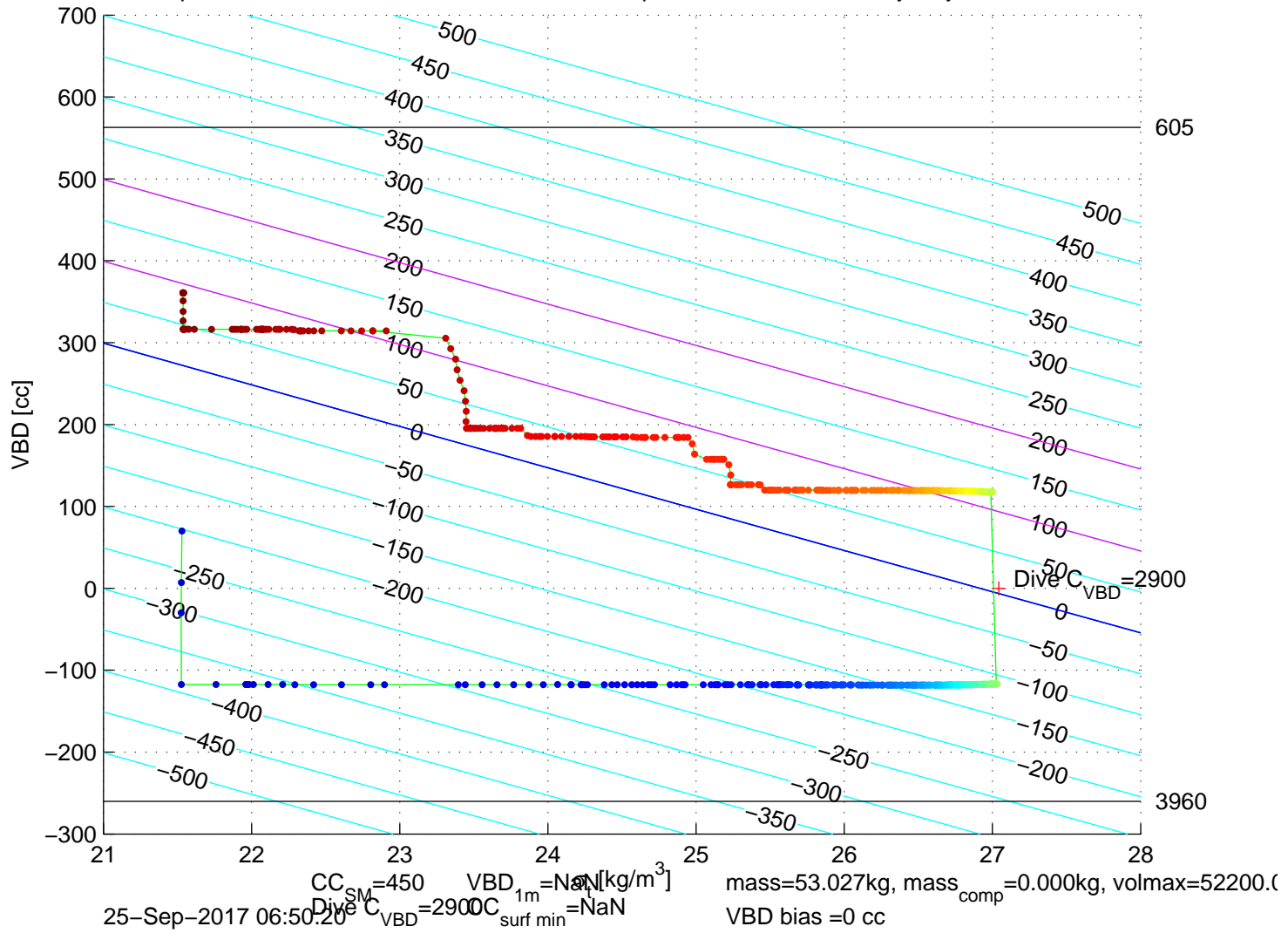
p6300586: SG630 Mission 7 Jul 2017 25-Sep-2017 08:17:33Z – buoyancy contoured
