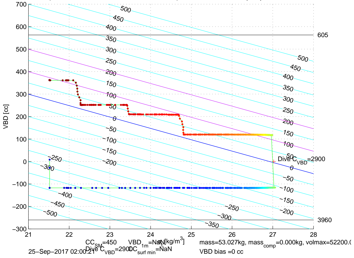
p6300584: SG630 Mission 7 Jul 2017 25-Sep-2017 03:38:46Z – buoyancy contoured
