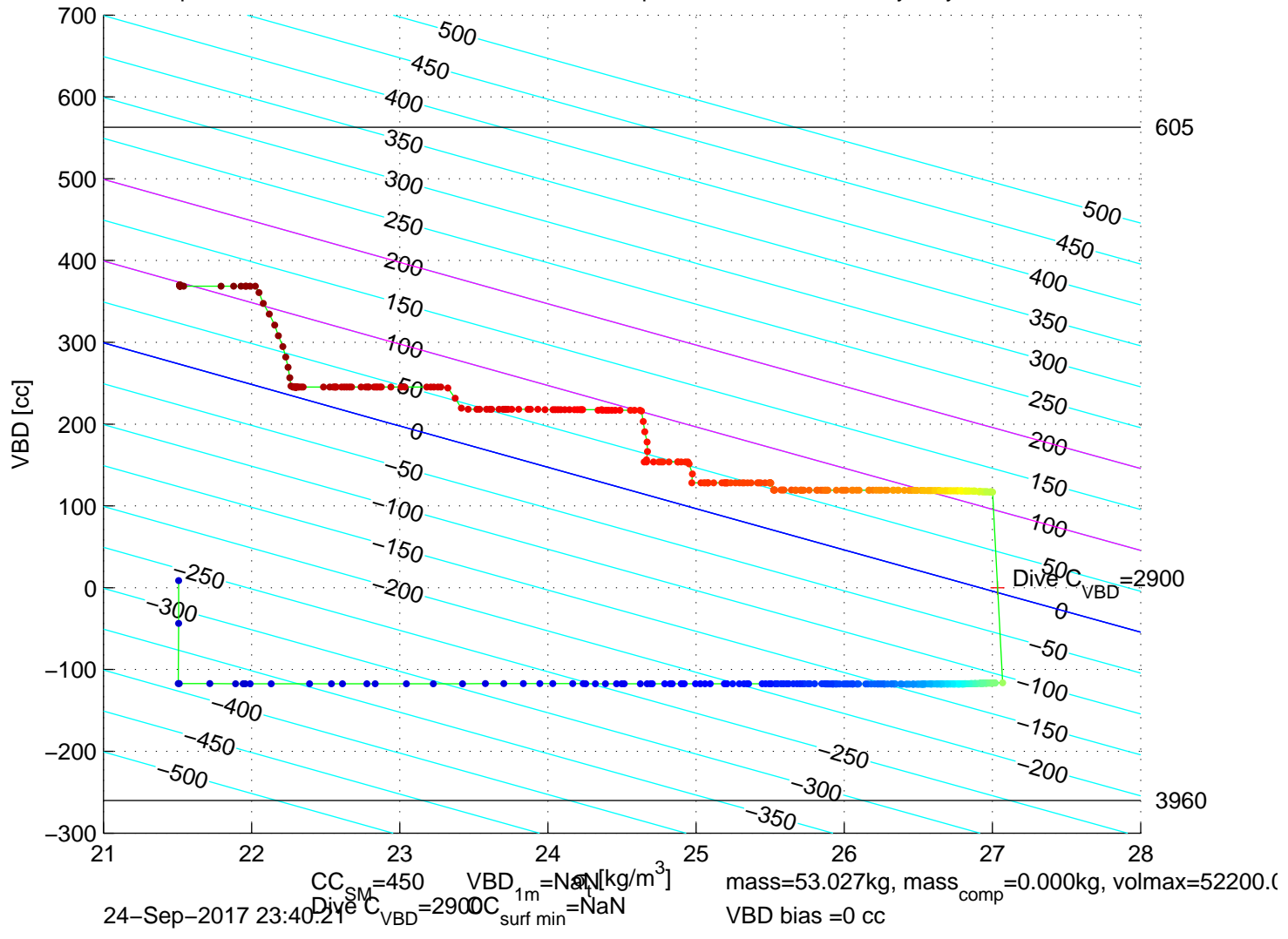
p6300583: SG630 Mission 7 Jul 2017 25-Sep-2017 01:13:27Z – buoyancy contoured
