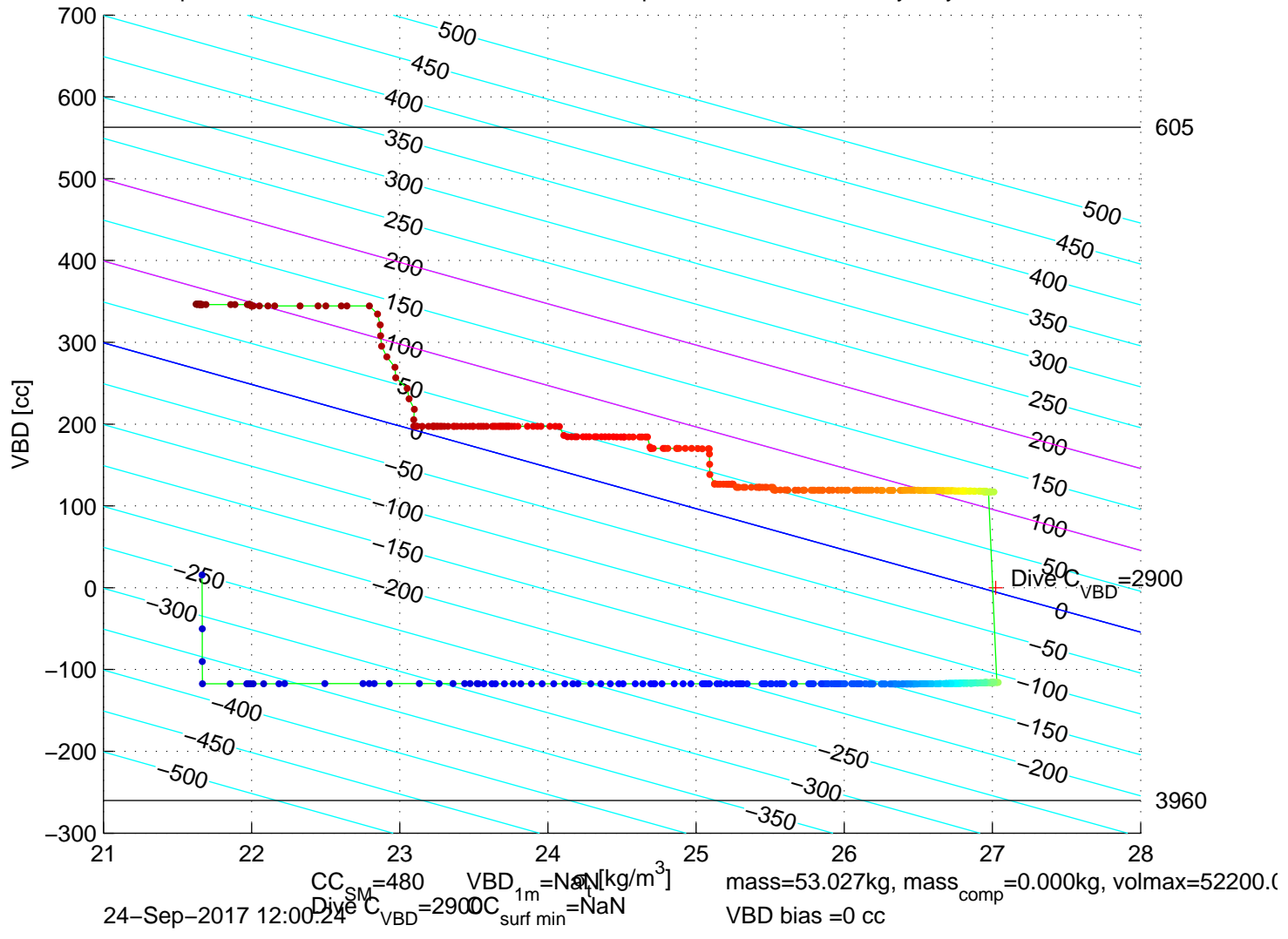
p6300578: SG630 Mission 7 Jul 2017 24-Sep-2017 13:17:13Z – buoyancy contoured
