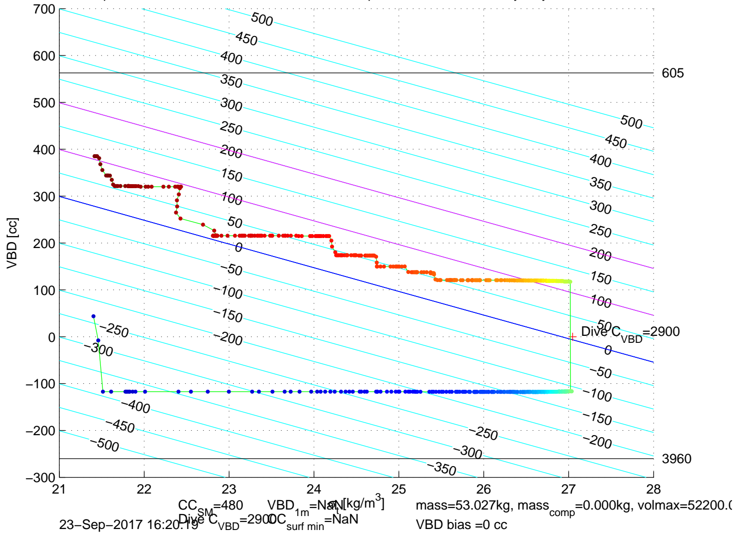
p6300570: SG630 Mission 7 Jul 2017 23-Sep-2017 17:45:18Z – buoyancy contoured
