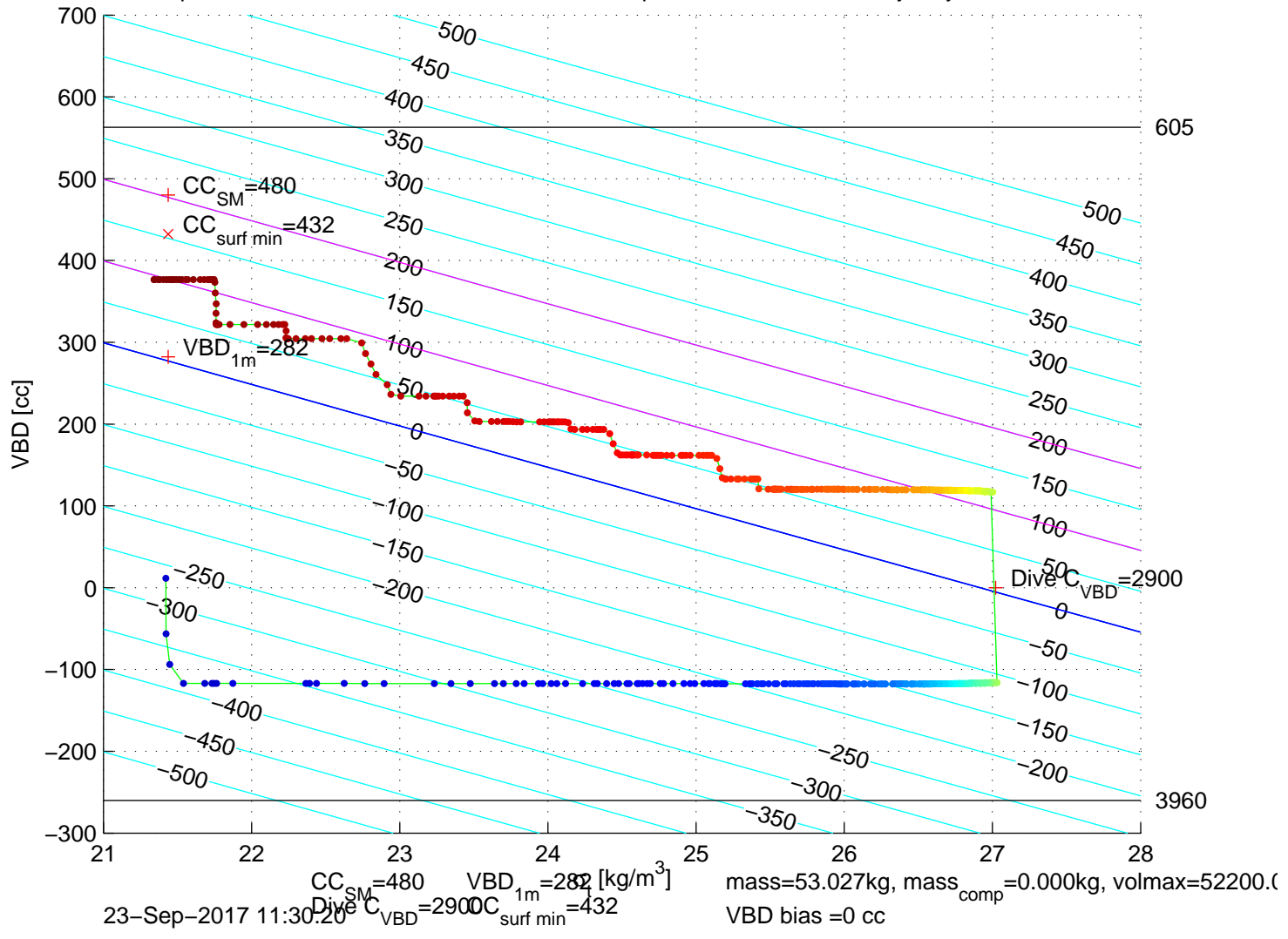
p6300568: SG630 Mission 7 Jul 2017 23-Sep-2017 13:04:36Z – buoyancy contoured
