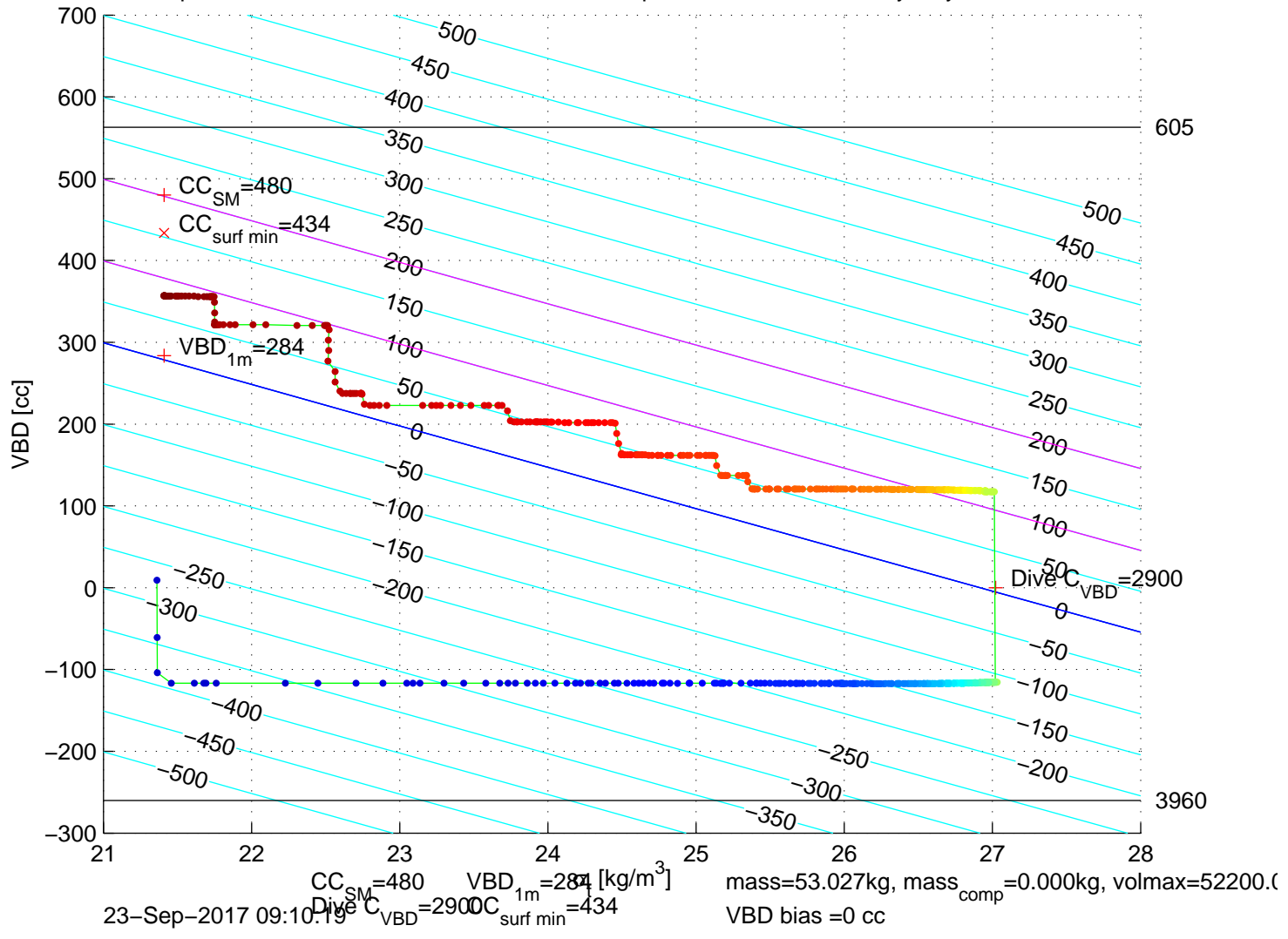
p6300567: SG630 Mission 7 Jul 2017 23-Sep-2017 10:42:43Z – buoyancy contoured
