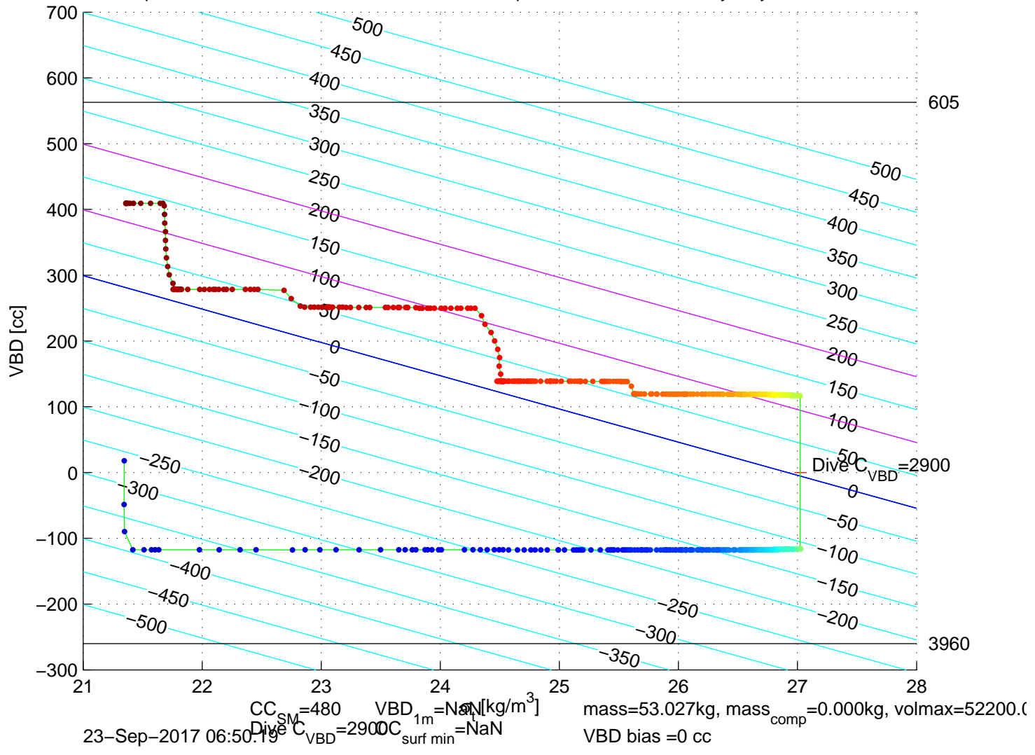
p6300566: SG630 Mission 7 Jul 2017 23-Sep-2017 08:19:47Z – buoyancy contoured
