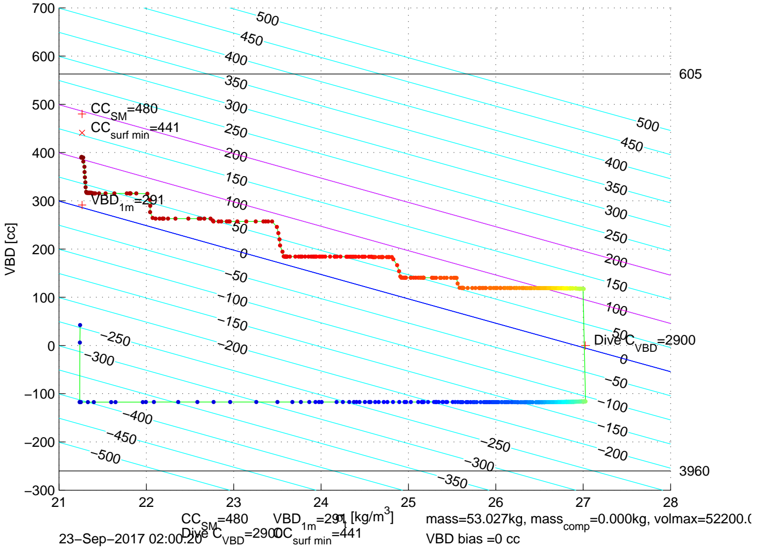
p6300564: SG630 Mission 7 Jul 2017 23-Sep-2017 03:09:09Z – buoyancy contoured
