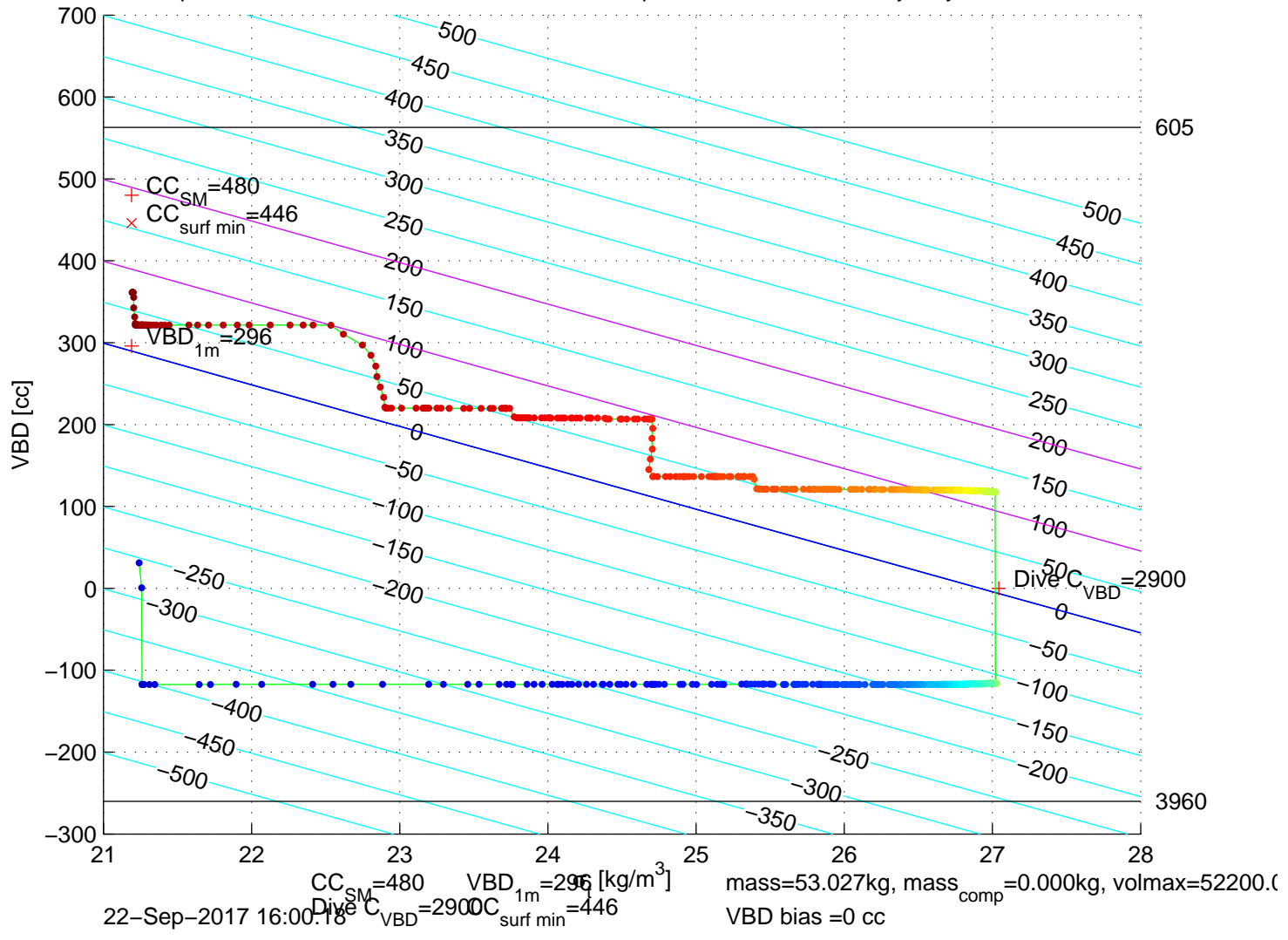
p6300560: SG630 Mission 7 Jul 2017 22-Sep-2017 17:35:25Z – buoyancy contoured
