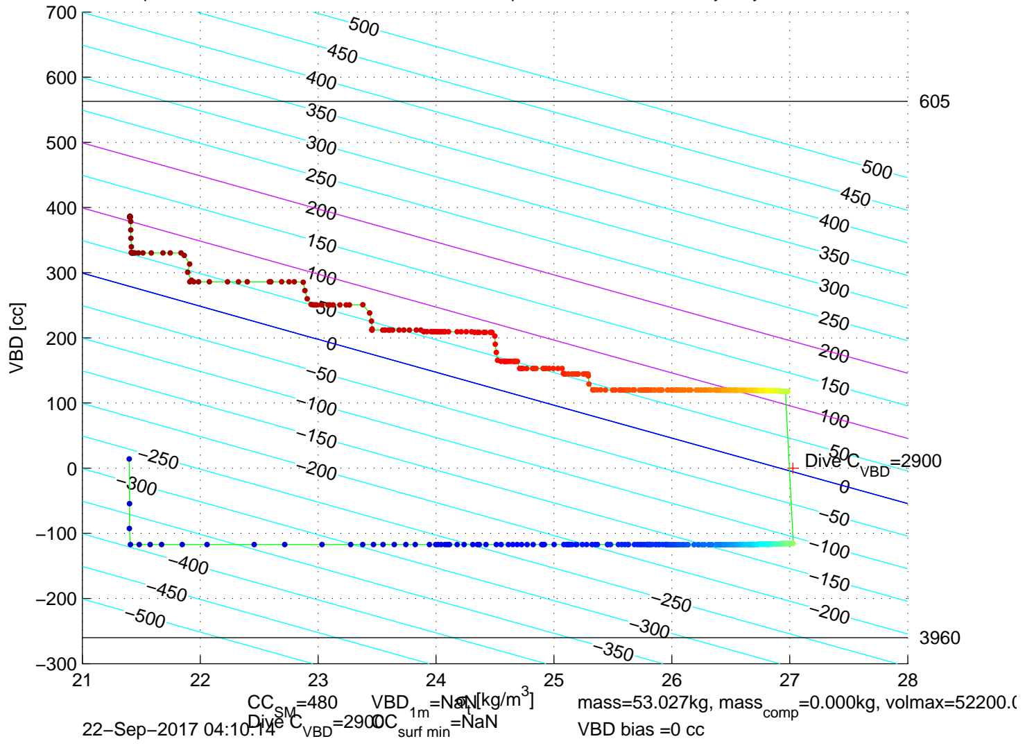
p6300555: SG630 Mission 7 Jul 2017 22-Sep-2017 05:49:52Z – buoyancy contoured
