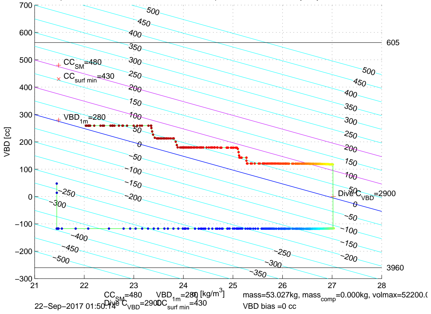
p6300554: SG630 Mission 7 Jul 2017 22-Sep-2017 03:29:24Z – buoyancy contoured
