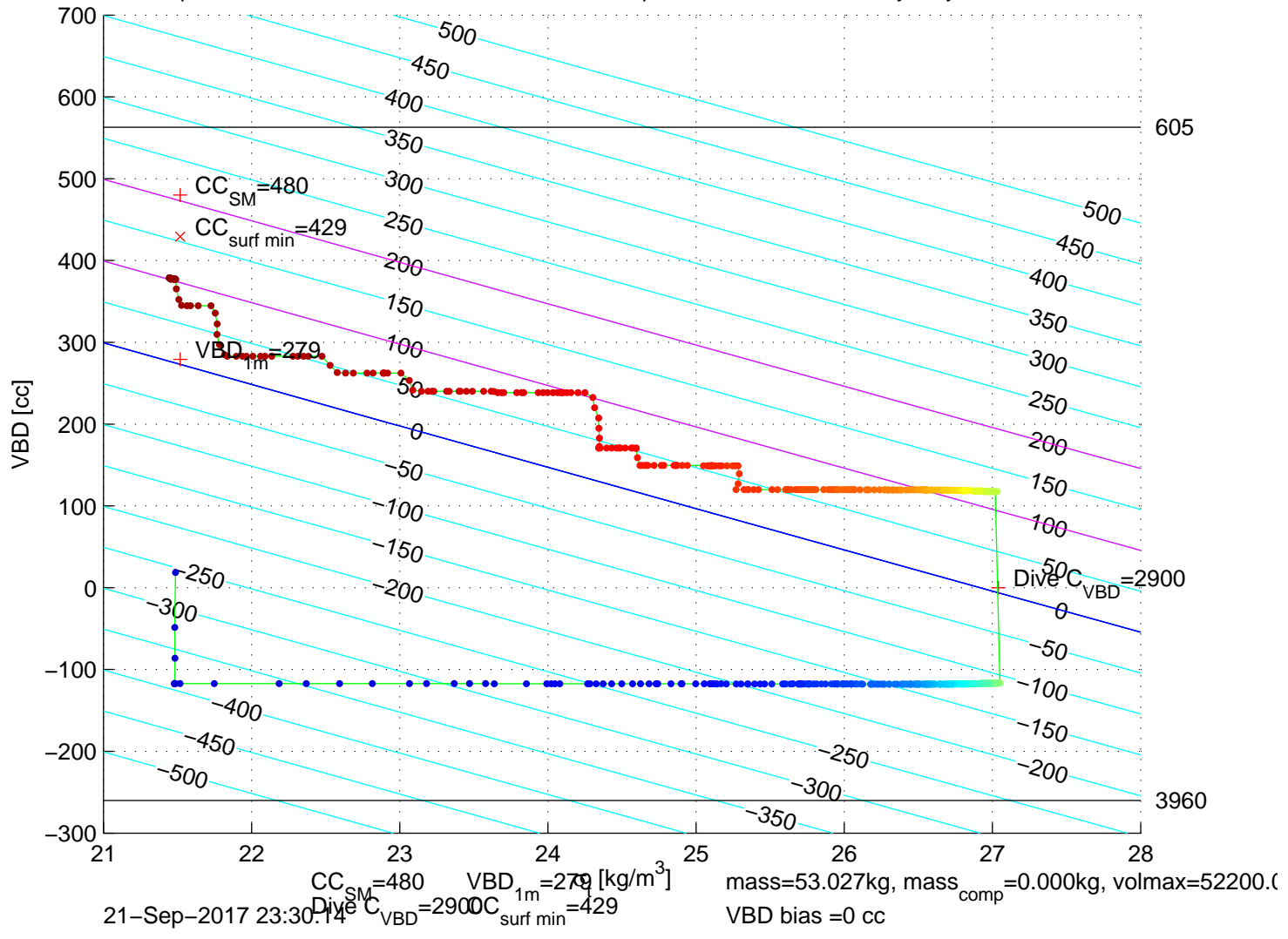
p6300553: SG630 Mission 7 Jul 2017 22-Sep-2017 01:11:24Z – buoyancy contoured
