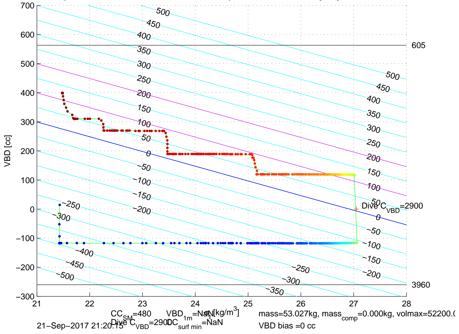
p6300552: SG630 Mission 7 Jul 2017 21-Sep-2017 22:51:35Z – buoyancy contoured
