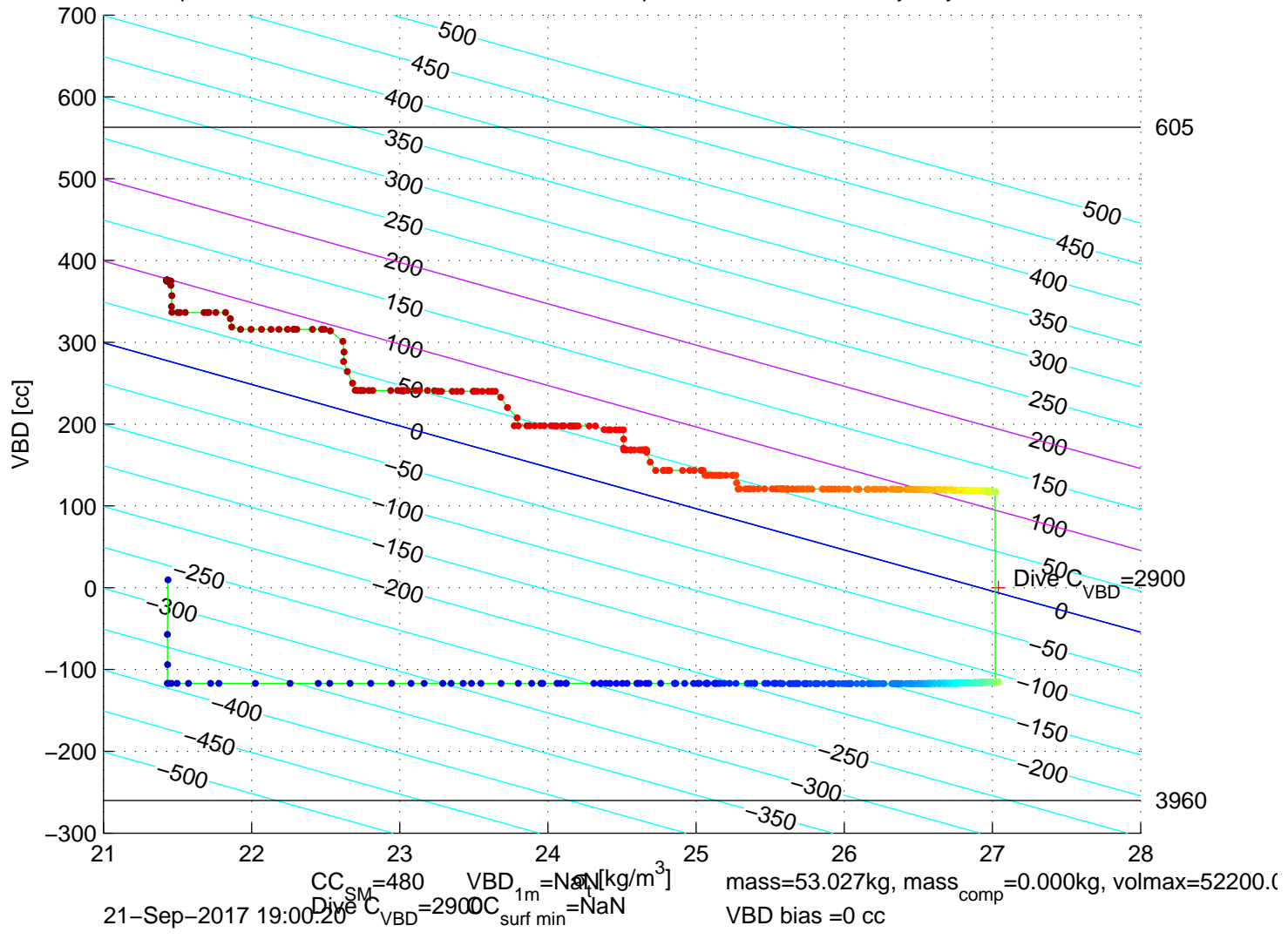
p6300551: SG630 Mission 7 Jul 2017 21-Sep-2017 20:29:59Z – buoyancy contoured
