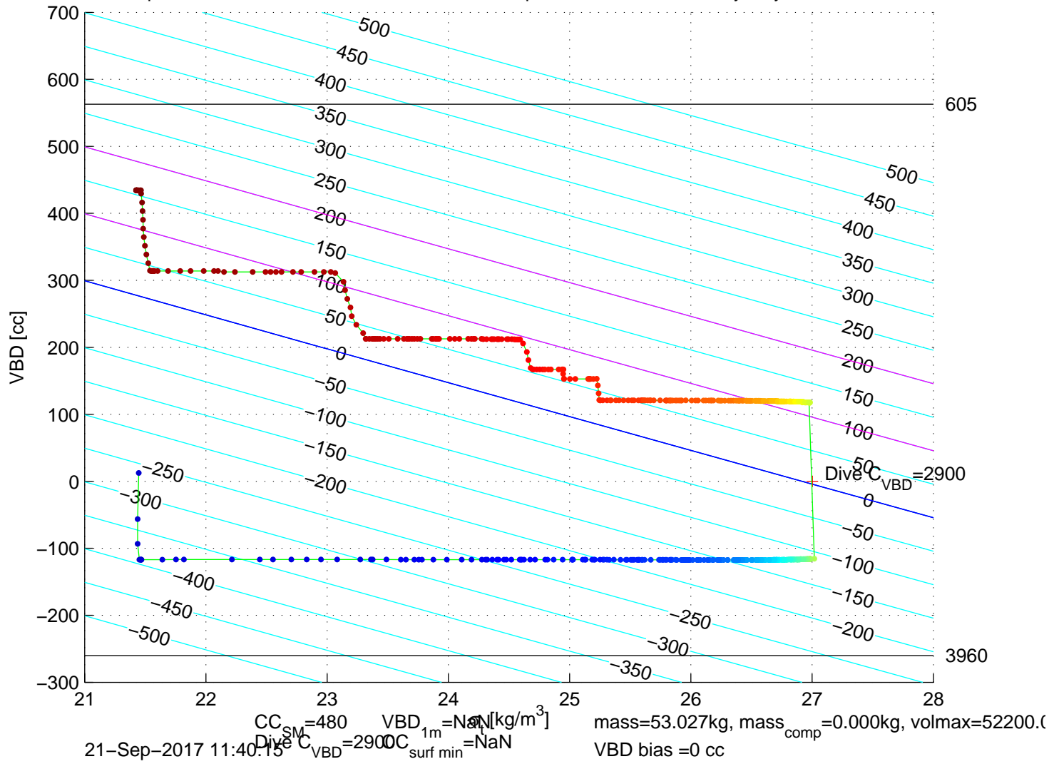
p6300548: SG630 Mission 7 Jul 2017 21-Sep-2017 13:16:48Z – buoyancy contoured
