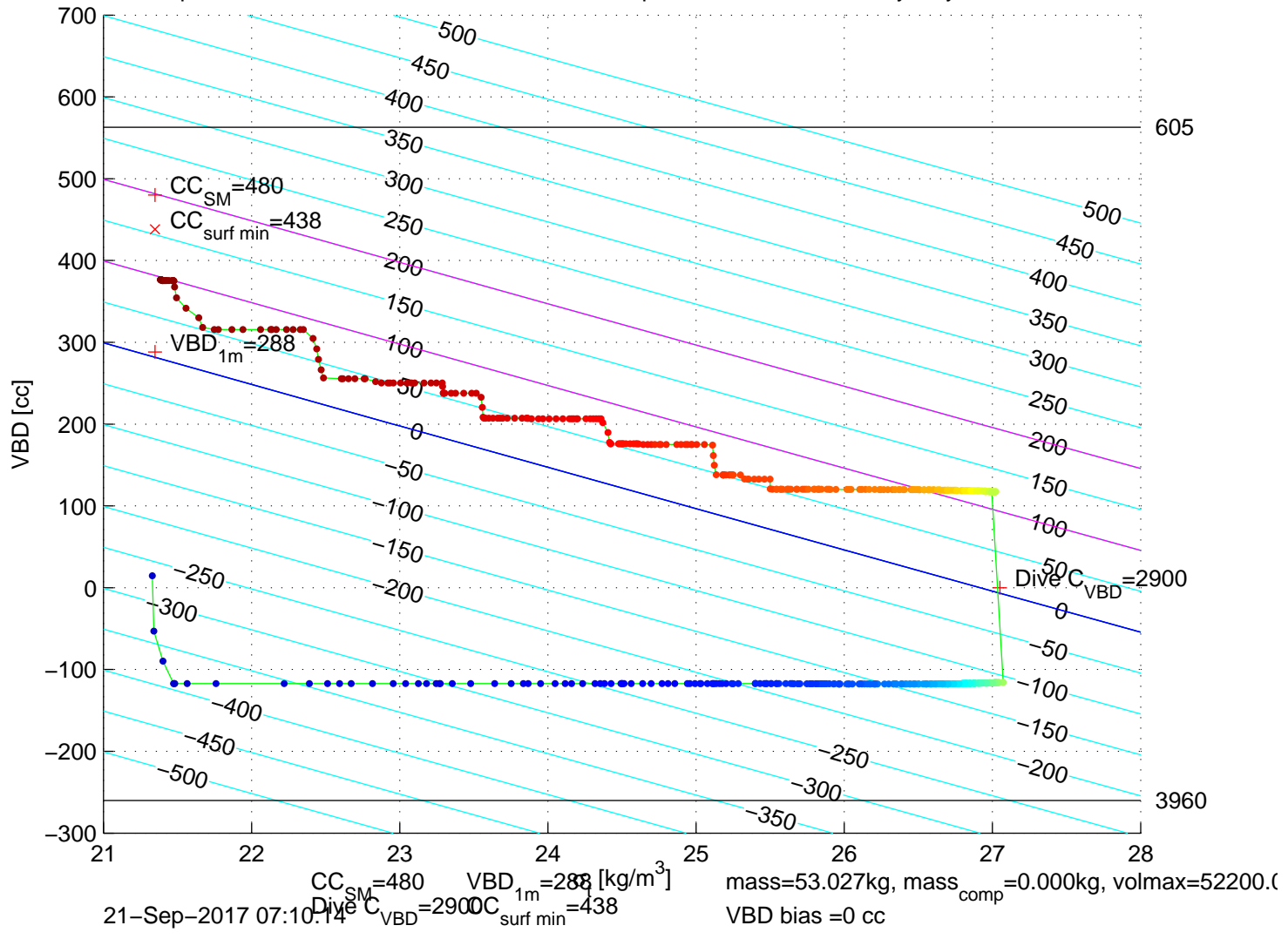
p6300546: SG630 Mission 7 Jul 2017 21-Sep-2017 08:43:01Z – buoyancy contoured
