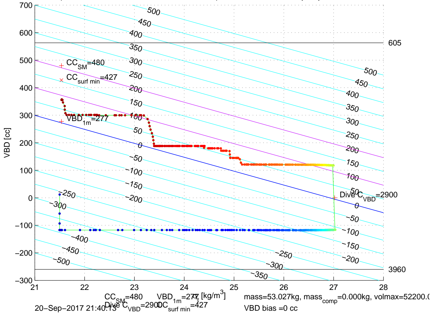
p6300542: SG630 Mission 7 Jul 2017 20-Sep-2017 23:15:34Z – buoyancy contoured
