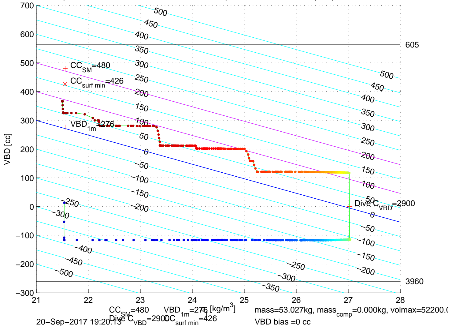
p6300541: SG630 Mission 7 Jul 2017 20-Sep-2017 20:57:50Z – buoyancy contoured
