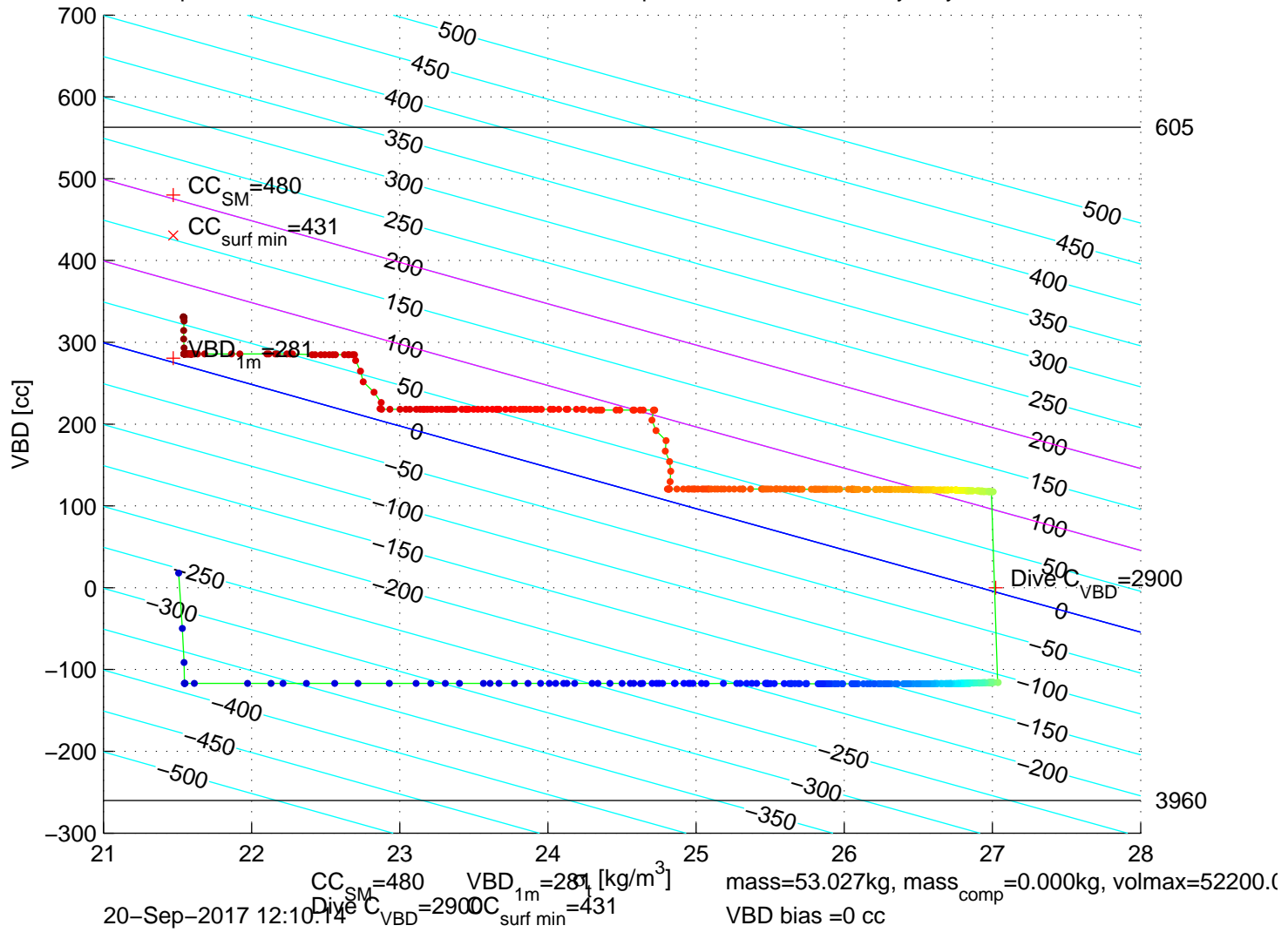
p6300538: SG630 Mission 7 Jul 2017 20-Sep-2017 13:38:26Z – buoyancy contoured
