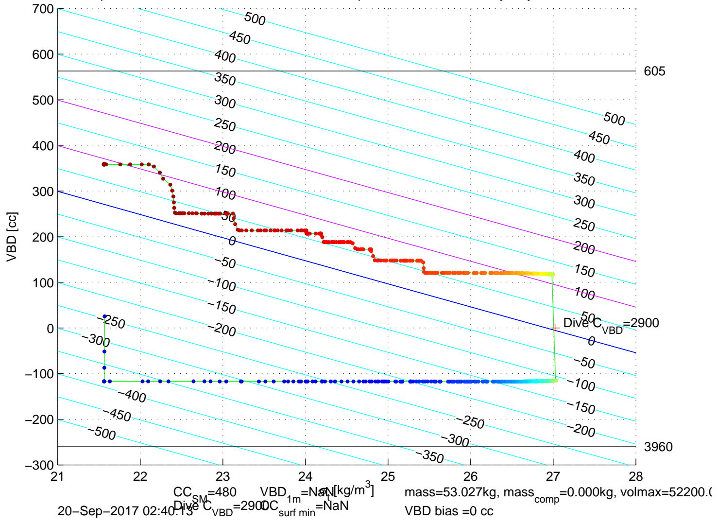
p6300534: SG630 Mission 7 Jul 2017 20-Sep-2017 04:05:45Z – buoyancy contoured
