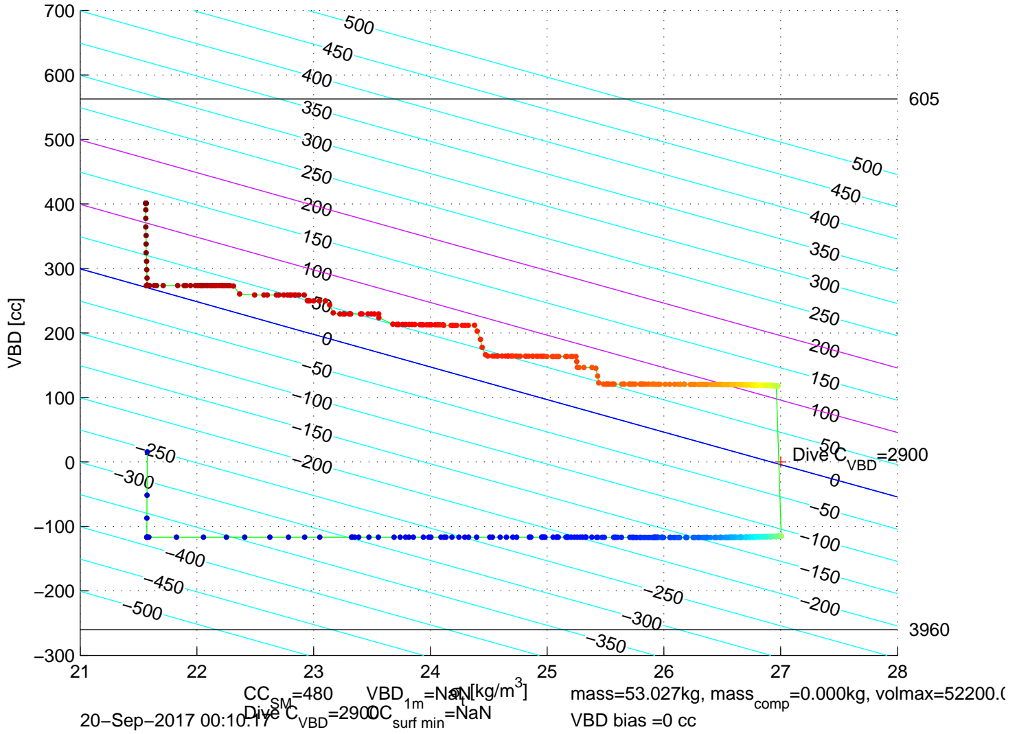
p6300533: SG630 Mission 7 Jul 2017 20-Sep-2017 01:36:39Z – buoyancy contoured
