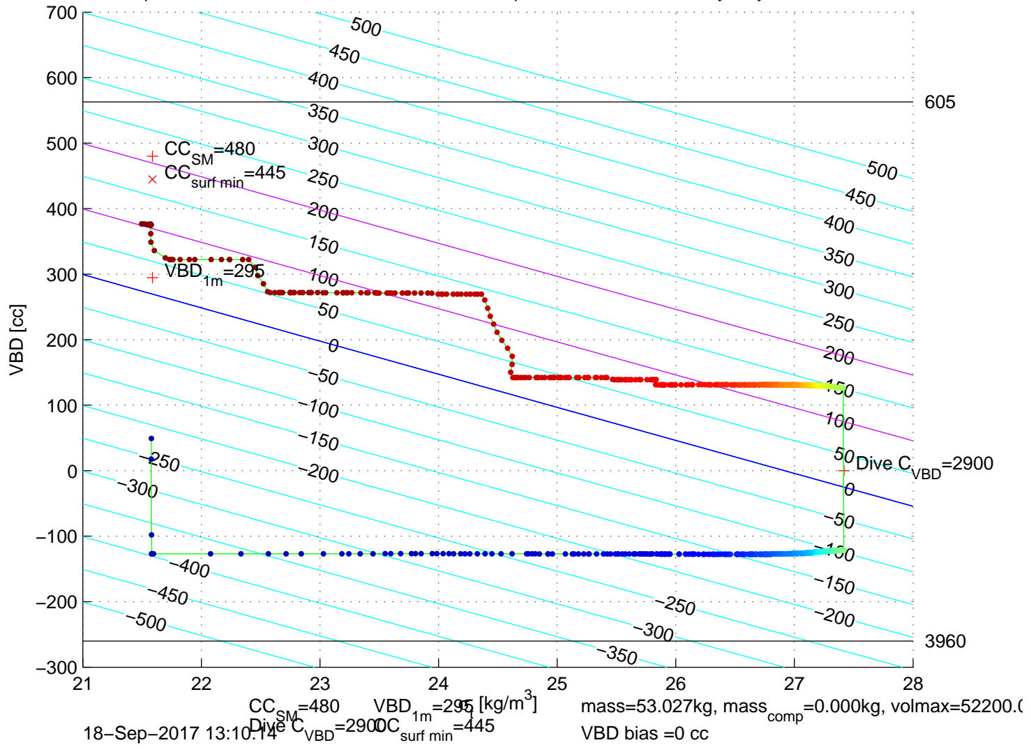
p6300519: SG630 Mission 7 Jul 2017 18-Sep-2017 13:09:48Z – buoyancy contoured
