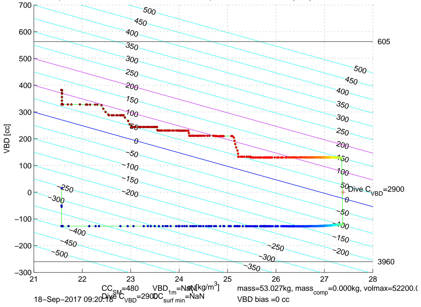
p6300518: SG630 Mission 7 Jul 2017 18-Sep-2017 09:03:53Z – buoyancy contoured
