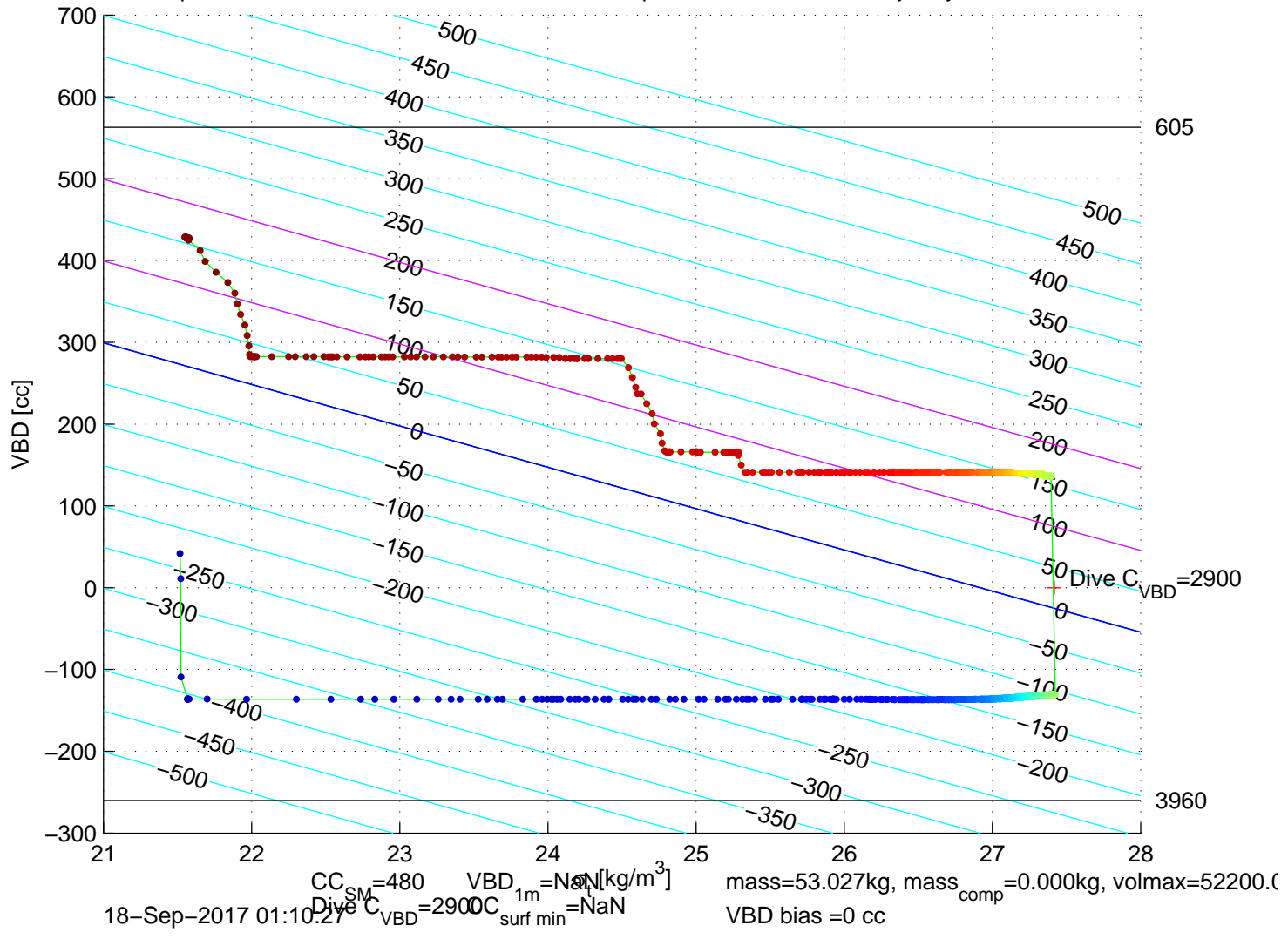
p6300516: SG630 Mission 7 Jul 2017 18-Sep-2017 01:08:01Z – buoyancy contoured
