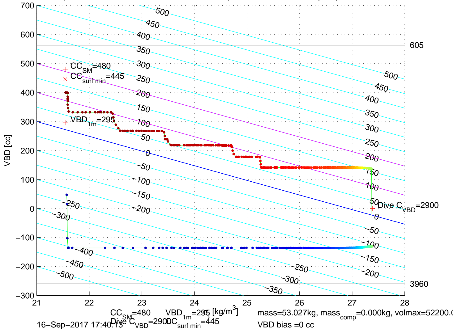
p6300508: SG630 Mission 7 Jul 2017 16-Sep-2017 17:40:03Z – buoyancy contoured
