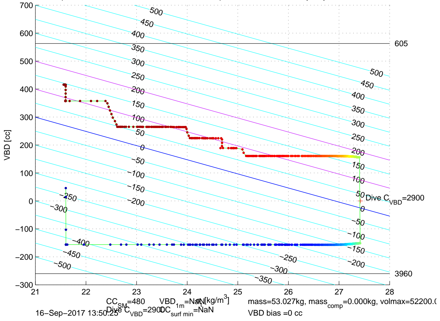
p6300507: SG630 Mission 7 Jul 2017 16-Sep-2017 14:02:03Z – buoyancy contoured
